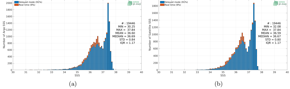
Figure 2: Histograms of SSS from Argo (a) and Aquarius SSS L4 OI v5 - Weekly (IPRC) (b) considering all match-up pairs per bins of 0.1 over the Amazon and Orinoco river plumes Pi-MEP region and for the full satellite product period.
