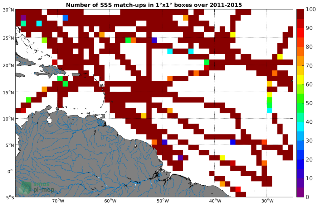
Figure 4: Number of SSS match-ups between TSG-SAMOS SSS and the Aquarius-L4-IPRC-V5-MONTHLY SSS product for the Amazon and Orinoco river plumes Pi-MEP region over 1^\circ \times 1^\circ boxes and for the full satellite product period.
