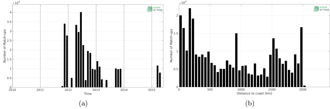
Figure 1: Number of match-ups between TSG-SAMOS and Aquarius-L4-IPRC-V5-MONTHLY SSS as a function of time (a) and as function of the distance to coast (b) over the Amazon and Orinoco river plumes Pi-MEP region and for the full satellite product period.
