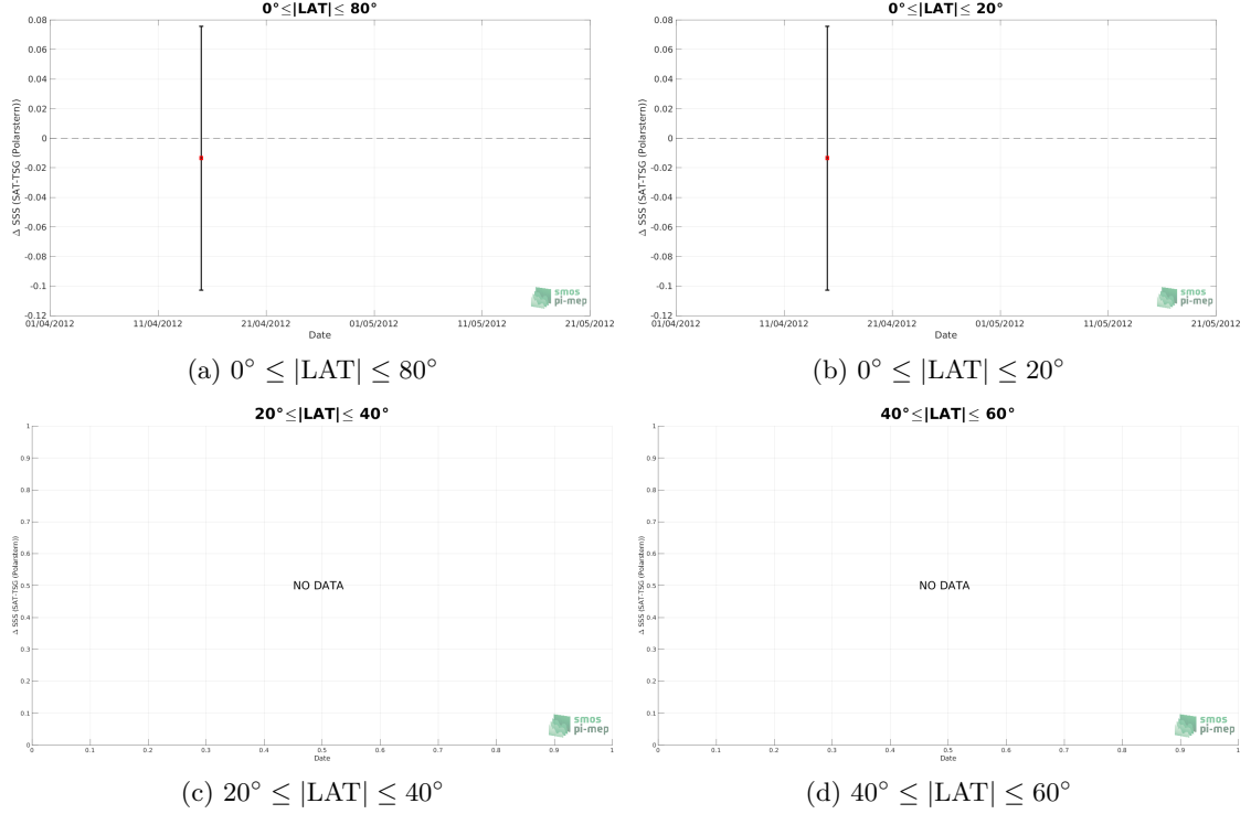
Figure 10: Monthly median (red curves) of \Delta\text{SSS} (Satellite - TSG (Polarstern)) and \pm 1 Std (black vertical thick bars) as function of time for all the collected Pi-MEP match-up pairs estimated over the Amazon and Orinoco river plumes Pi-MEP region and for the full satellite product period are shown for different latitude bands: (a) 80^{\circ}\text{S}-80^{\circ}\text{N} , (b) 20^{\circ}\text{S}-20^{\circ}\text{N} , (c) 40^{\circ}\text{S}-20^{\circ}\text{S} and 20^{\circ}\text{N}-40^{\circ}\text{N} and (d) 60^{\circ}\text{S}-40^{\circ}\text{S} and 40^{\circ}\text{N}-60^{\circ}\text{N} .
