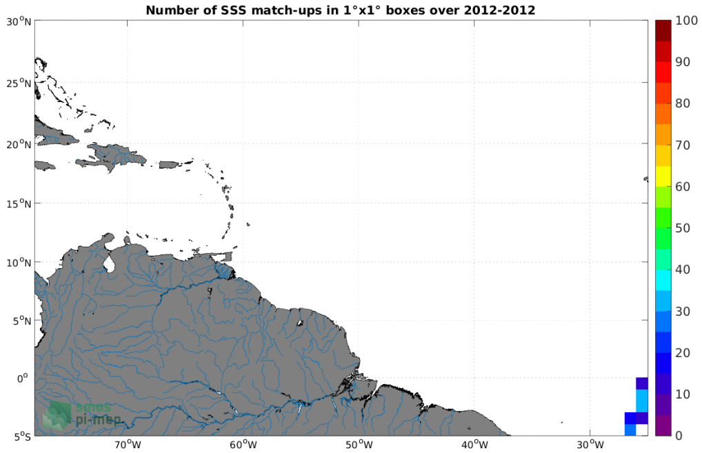
Figure 4: Number of SSS match-ups between TSG (Polarstern) SSS and the Aquarius SSS L4 OI v5 - Monthly (IPRC) SSS product for the Amazon and Orinoco river plumes Pi-MEP region over 1°x1° boxes and for the full satellite product period.
