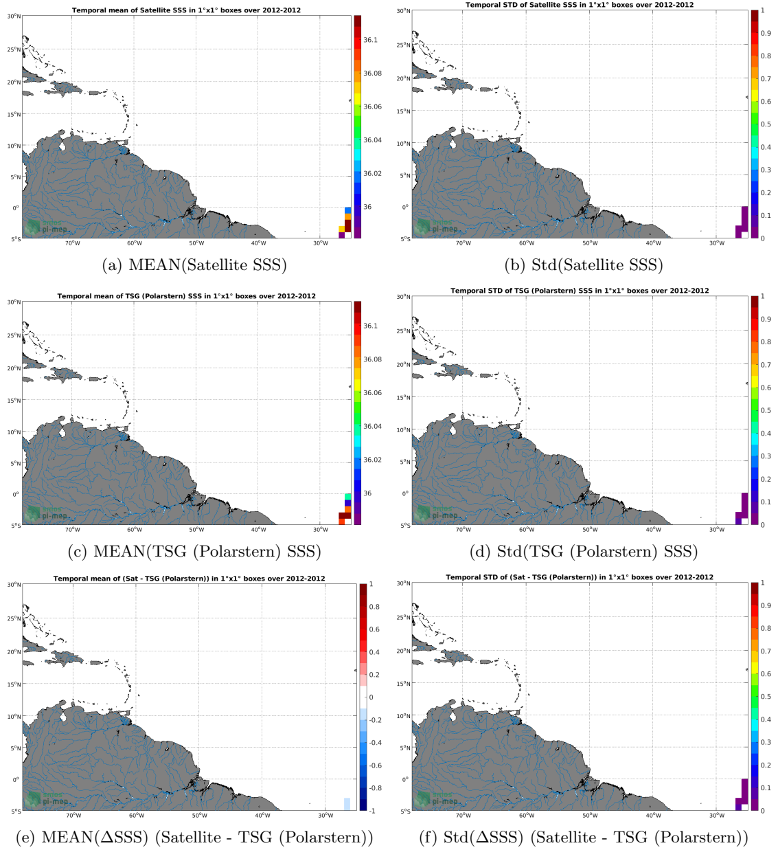
Figure 6: Temporal mean (left) and Std (right) of SSS from Aquarius SSS L4 OI v5 - Monthly (IPRC) (top), TSG (Polarstern) (middle), and of \Delta SSS (Satellite - TSG (Polarstern)). Only match-up pairs are used to generate these maps.
