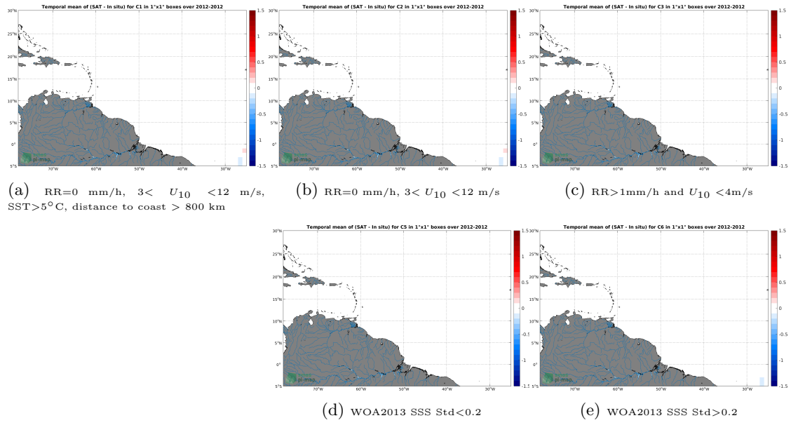
Figure 12: Temporal mean gridded over spatial boxes of size 1^\circ \times 1^\circ of \Delta SSS (Aquarius SSS L4 OI v5 - Monthly (IPRC) - TSG (Polarstern)) for 5 different subdatasets corresponding to: RR=0 mm/h, 3 < U_{10} < 12 m/s, SST > 5^\circ\text{C} , distance to coast > 800 km (a), RR=0 mm/h, 3 < U_{10} < 12 m/s (b), RR > 1 mm/h and U_{10} < 4 m/s (c), WOA2013 SSS Std < 0.2 (d), WOA2013 SSS Std > 0.2 (e).
