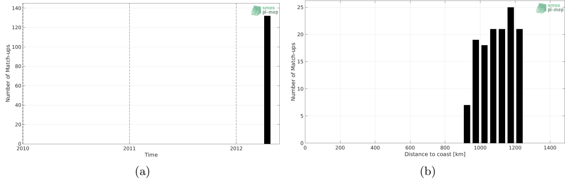
Figure 1: Number of match-ups between TSG (Polarstern) and Aquarius SSS L4 OI v5 - Monthly (IPRC) SSS as a function of time (a) and as function of the distance to coast (b) over the Amazon and Orinoco river plumes Pi-MEP region and for the full satellite product period.
