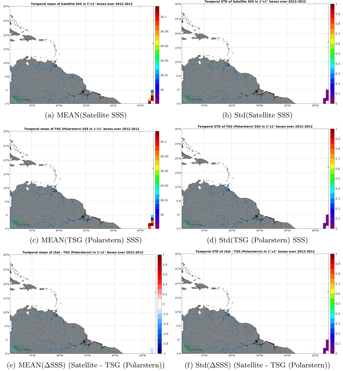
Figure 6: Temporal mean (left) and Std (right) of SSS from Aquarius SSS L4 OI v5 - Monthly (IPRC) (top), TSG (Polarstern) (middle), and of \Delta SSS (Satellite - TSG (Polarstern)). Only match-pairs are used to generate these maps.
