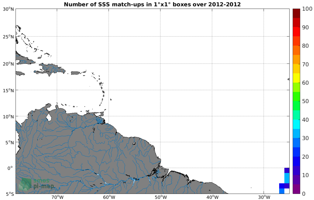
Figure 4: Number of SSS match-ups between TSG (Polarstern) SSS and the Aquarius SSS L4 OI v5 - Monthly (IPRC) SSS product for the Amazon and Orinoco river plumes Pi-MEP region over 1^\circ \times 1^\circ boxes and for the full satellite product period.
