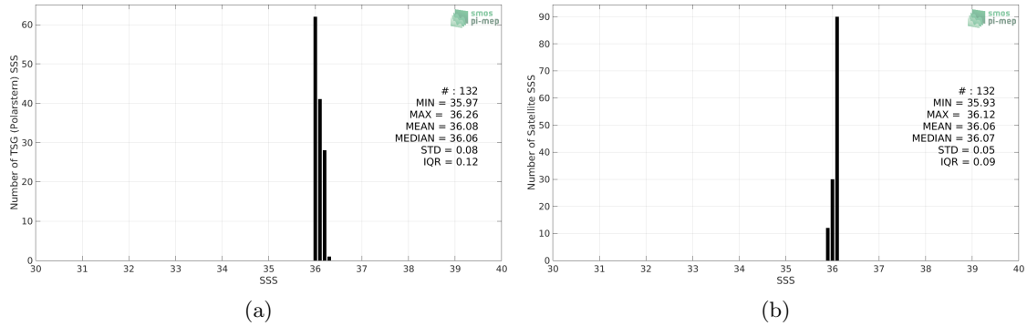
Figure 2: Histograms of SSS from TSG (Polarstern) (a) and Aquarius SSS L4 OI v5 - Monthly (IPRC) (b) considering all match-up pairs per bins of 0.1 over the Amazon and Orinoco river plumes Pi-MEP region and for the full satellite product period.
