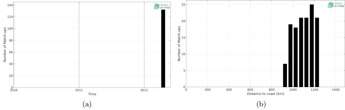
Figure 1: Number of match-ups between TSG-POLARSTERN and Aquarius-L4-IPRC-V5-MONTHLY SSS as a function of time (a) and as function of the distance to coast (b) over the Amazon and Orinoco river plumes Pi-MEP region and for the full satellite product period.
