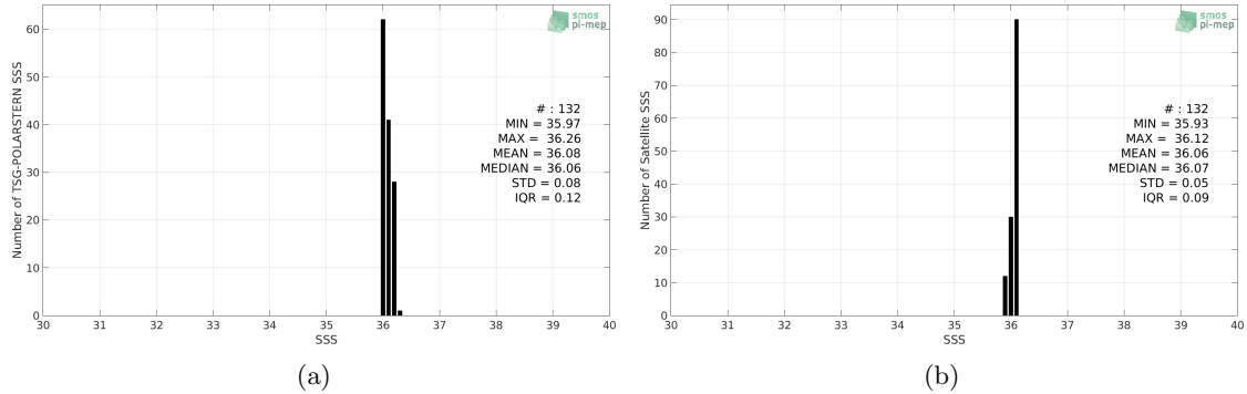
Figure 2: Histograms of SSS from TSG-POLARSTERN (a) and Aquarius-L4-IPRC-V5-MONTHLY (b) considering all match-up pairs per bins of 0.1 over the Amazon and Orinoco river plumes Pi-MEP region and for the full satellite product period.
