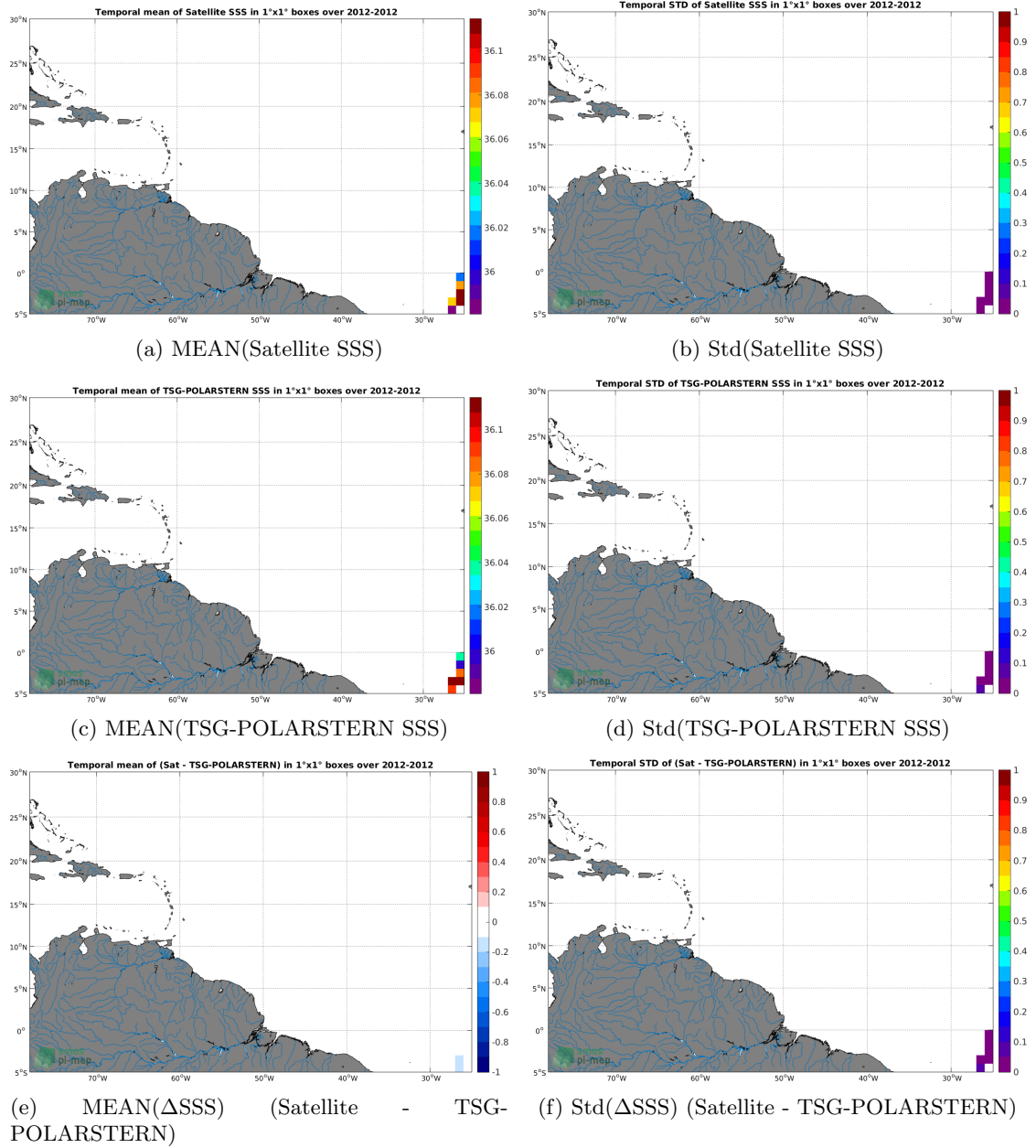
Figure 6: Temporal mean (left) and Std (right) of SSS from Aquarius-L4-IPRC-V5-MONTHLY (top), TSG-POLARSTERN (middle), and of \Delta SSS (Satellite - TSG-POLARSTERN). Only match-up pairs are used to generate these maps.
