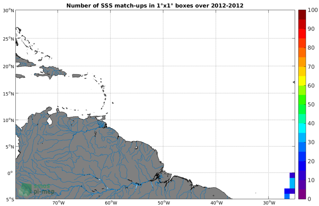
Figure 4: Number of SSS match-ups between TSG-POLARSTERN SSS and the Aquarius-L4-IPRC-V5-MONTHLY SSS product for the Amazon and Orinoco river plumes Pi-MEP region over 1^\circ \times 1^\circ boxes and for the full satellite product period.
