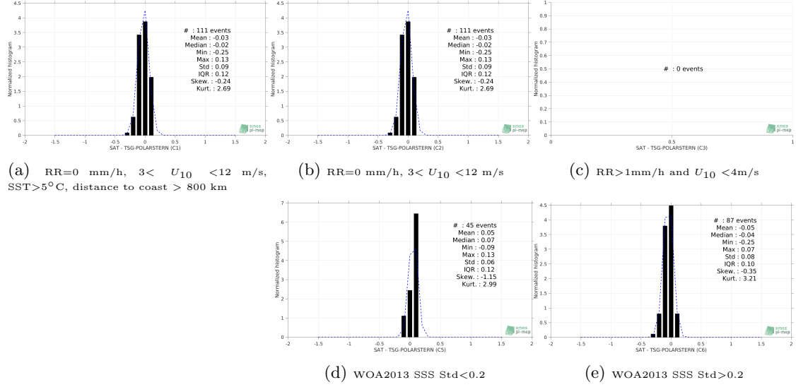
Figure 13: Normalized histogram of \Delta\text{SSS} (Aquarius-L4-IPRC-V5-MONTHLY - TSG-POLARSTERN) for 5 different subdatasets corresponding to: RR=0 mm/h, 3 < U_{10} < 12 m/s, SST > 5^\circ\text{C} , distance to coast > 800 km (a), RR=0 mm/h, 3 < U_{10} < 12 m/s (b), RR > 1\text{mm/h} and U_{10} < 4\text{m/s} (c), WOA2013 SSS Std <0.2 (d), WOA2013 SSS Std >0.2 (e).
