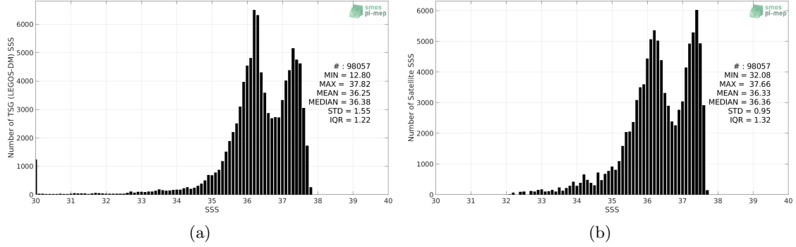
Figure 2: Histograms of SSS from TSG (LEGOS-DM) (a) and Aquarius SSS L4 OI v5 - Monthly (IPRC) (b) considering all match-up pairs per bins of 0.1 over the Amazon and Orinoco river plumes Pi-MEP region and for the full satellite product period.
