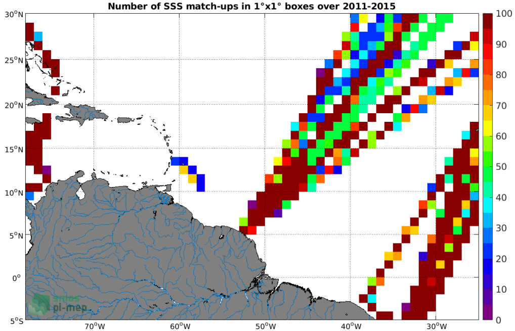
Figure 4: Number of SSS match-ups between TSG (LEGOS-DM) SSS and the Aquarius SSS L4 OI v5 - Monthly (IPRC) SSS product for the Amazon and Orinoco river plumes Pi-MEP region over 1^\circ \times 1^\circ boxes and for the full satellite product period.
