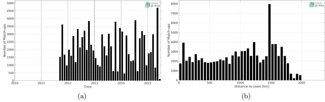
Figure 1: Number of match-ups between TSG (LEGOS-DM) and Aquarius SSS L4 OI v5 - Monthly (IPRC) SSS as a function of time (a) and as function of the distance to coast (b) over the Amazon and Orinoco river plumes Pi-MEP region and for the full satellite product period.
