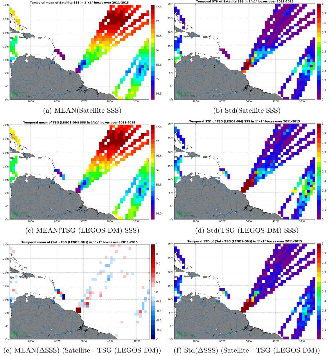
Figure 6: Temporal mean (left) and Std (right) of SSS from Aquarius SSS L4 OI v5 - Monthly (IPRC) (top), TSG (LEGOS-DM) (middle), and of \Delta SSS (Satellite - TSG (LEGOS-DM)). Only match-pairs are used to generate these maps.
