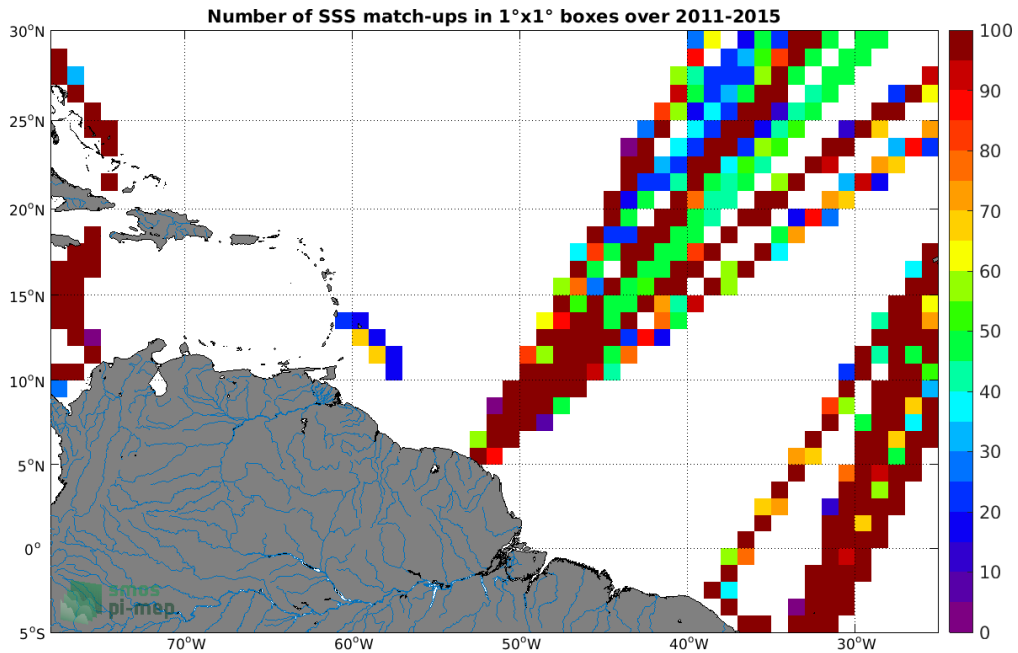
Figure 4: Number of SSS match-ups between TSG (LEGOS-DM) SSS and the Aquarius SSS L4 OI v5 - Monthly (IPRC) SSS product for the Amazon and Orinoco river plumes Pi-MEP region over 1°x1° boxes and for the full satellite product period.
