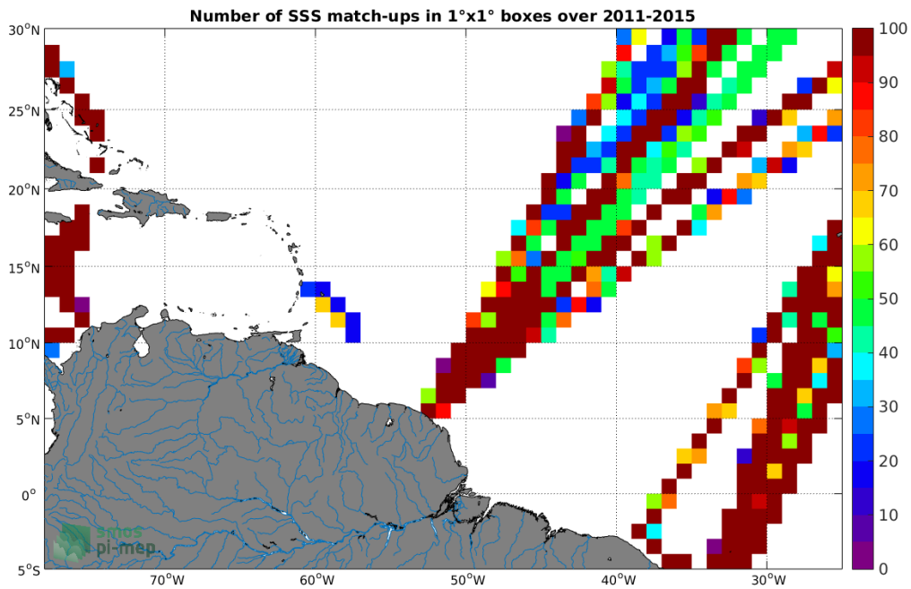
Figure 4: Number of SSS match-ups between TSG-LEGOS-DM SSS and the Aquarius-L4-IPRC-V5-MONTHLY SSS product for the Amazon and Orinoco river plumes Pi-MEP region over 1^\circ \times 1^\circ boxes and for the full satellite product period.
