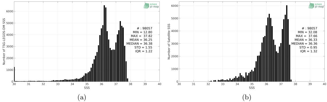
Figure 2: Histograms of SSS from TSG-LEGOS-DM (a) and Aquarius-L4-IPRC-V5-MONTHLY (b) considering all match-up pairs per bins of 0.1 over the Amazon and Orinoco river plumes Pi-MEP region and for the full satellite product period.
