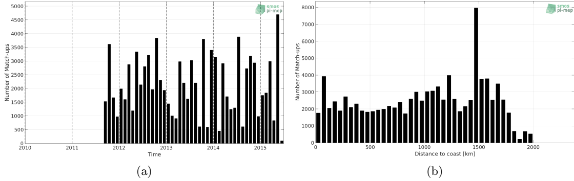
Figure 1: Number of match-ups between TSG-LEGOS-DM and Aquarius-L4-IPRC-V5-MONTHLY SSS as a function of time (a) and as function of the distance to coast (b) over the Amazon and Orinoco river plumes Pi-MEP region and for the full satellite product period.
