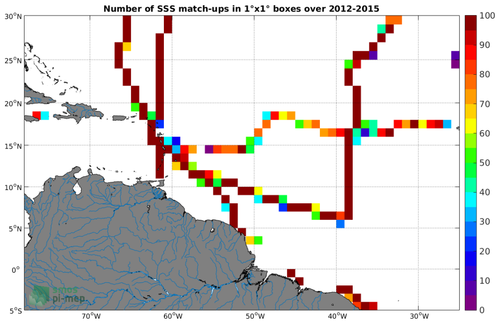
Figure 4: Number of SSS match-ups between TSG-GOSUD-Sailing-ship SSS and the Aquarius-L4-IPRC-V5-MONTHLY SSS product for the Amazon and Orinoco river plumes Pi-MEP region over 1^\circ \times 1^\circ boxes and for the full satellite product period.
