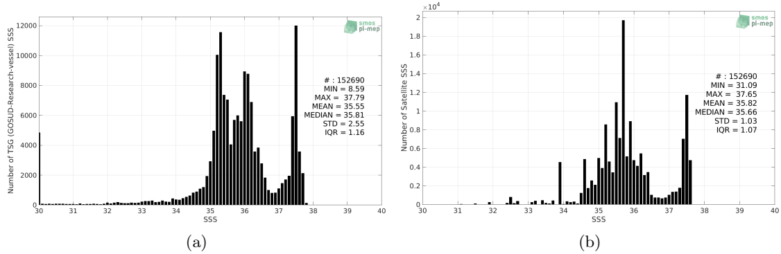
Figure 2: Histograms of SSS from TSG (GOSUD-Research-vessel) (a) and Aquarius SSS L4 OI v5 - Monthly (IPRC) (b) considering all match-up pairs per bins of 0.1 over the Amazon and Orinoco river plumes Pi-MEP region and for the full satellite product period.
