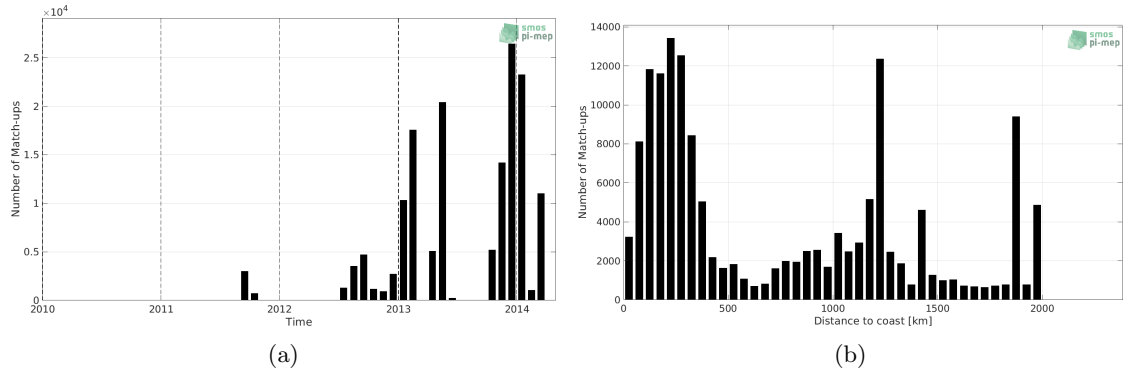
Figure 1: Number of match-ups between TSG (GOSUD-Research-vessel) and Aquarius SSS L4 OI v5 - Monthly (IPRC) SSS as a function of time (a) and as function of the distance to coast (b) over the Amazon and Orinoco river plumes Pi-MEP region and for the full satellite product period.
