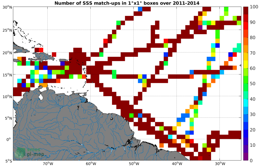
Figure 4: Number of SSS match-ups between TSG (GOSUD-Research-vessel) SSS and the Aquarius SSS L4 OI v5 - Monthly (IPRC) SSS product for the Amazon and Orinoco river plumes Pi-MEP region over 1^\circ \times 1^\circ boxes and for the full satellite product period.
