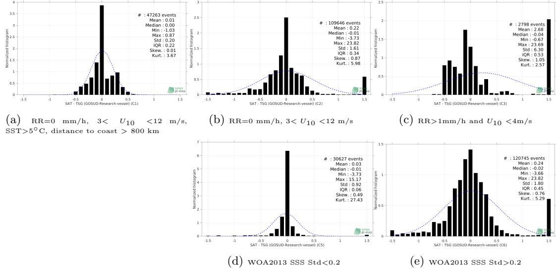
Figure 13: Normalized histogram of \Delta\text{SSS} (Aquarius SSS L4 OI v5 - Monthly (IPRC) - TSG (GOSUD-Research-vessel)) for 5 different subdatasets corresponding to: RR=0 mm/h, 3 < U_{10} < 12 m/s, SST>5°C, distance to coast > 800 km (a), RR=0 mm/h, 3 < U_{10} < 12 m/s (b), RR>1mm/h and U_{10} < 4 m/s (c), WOA2013 SSS Std<0.2 (d), WOA2013 SSS Std>0.2 (e).
