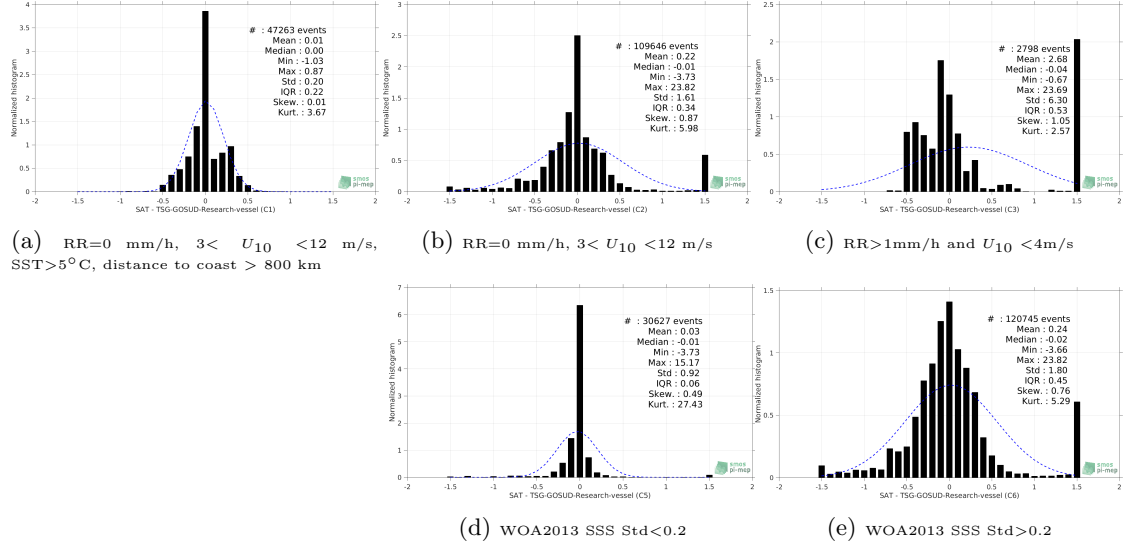
Figure 13: Normalized histogram of \Delta SSS (Aquarius-L4-IPRC-V5-MONTHLY - TSG-GOSUD-Research-vessel) for 5 different subdatasets corresponding to: RR=0 mm/h, 3 < U_{10} < 12 m/s, SST>5°C, distance to coast > 800 km (a), RR=0 mm/h, 3 < U_{10} < 12 m/s (b), RR>1mm/h and U_{10} < 4 m/s (c), WOA2013 SSS Std<0.2 (d), WOA2013 SSS Std>0.2 (e).
