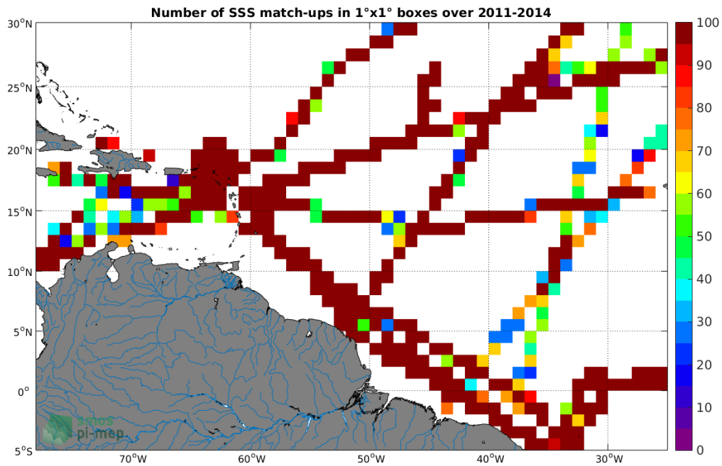
Figure 4: Number of SSS match-ups between TSG-GOSUD-Research-vessel SSS and the Aquarius-L4-IPRC-V5-MONTHLY SSS product for the Amazon and Orinoco river plumes Pi-MEP region over 1°x1° boxes and for the full satellite product period.
