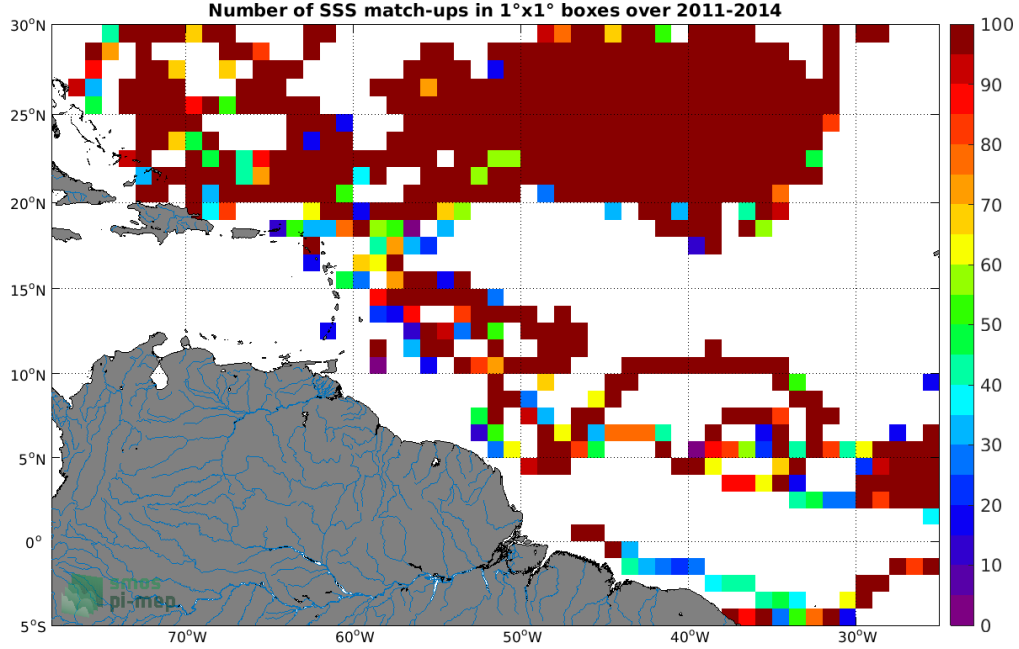
Figure 3: Number of SSS match-ups between Surface drifters SSS and the Aquarius SSS L4 OI v5 - Monthly (IPRC) SSS product for the Amazon and Orinoco river plumes Pi-MEP region over 1^\circ \times 1^\circ boxes and for the full satellite product period.
