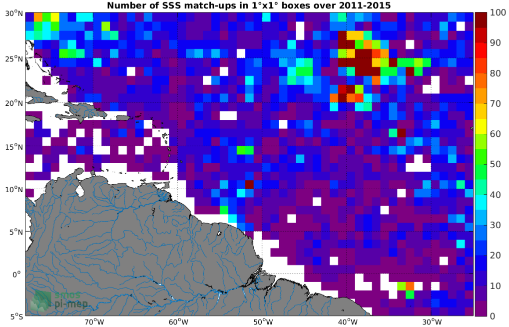
Figure 4: Number of SSS match-ups between Argo SSS and the Aquarius SSS L4 OI v5 - Monthly (IPRC) SSS product for the Amazon and Orinoco river plumes Pi-MEP region over 1^\circ \times 1^\circ boxes and for the full satellite product period.
