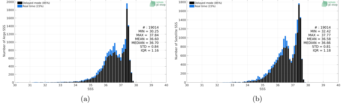
Figure 2: Histograms of SSS from Argo (a) and Aquarius SSS L4 OI v5 - Monthly (IPRC) (b) considering all match-up pairs per bins of 0.1 over the Amazon and Orinoco river plumes Pi-MEP region and for the full satellite product period.
