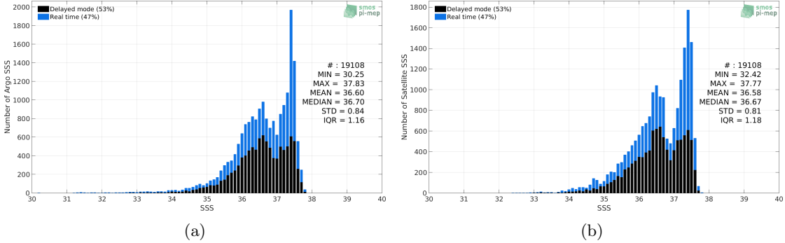
Figure 2: Histograms of SSS from Argo (a) and Aquarius-L4-IPRC-V5-MONTHLY (b) considering all match-up pairs per bins of 0.1 over the Amazon and Orinoco river plumes Pi-MEP region and for the full satellite product period.
