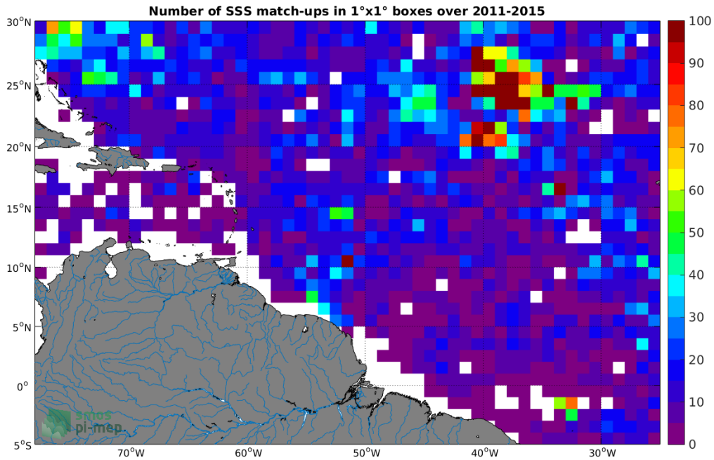
Figure 4: Number of SSS match-ups between Argo SSS and the Aquarius-L4-IPRC-V5-MONTHLY SSS product for the Amazon and Orinoco river plumes Pi-MEP region over 1^\circ \times 1^\circ boxes and for the full satellite product period.
