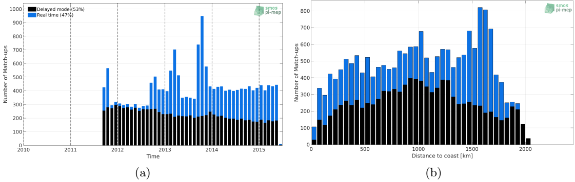
Figure 1: Number of match-ups between Argo and Aquarius-L4-IPRC-V5-MONTHLY SSS as a function of time (a) and as function of the distance to coast (b) over the Amazon and Orinoco river plumes Pi-MEP region and for the full satellite product period.
