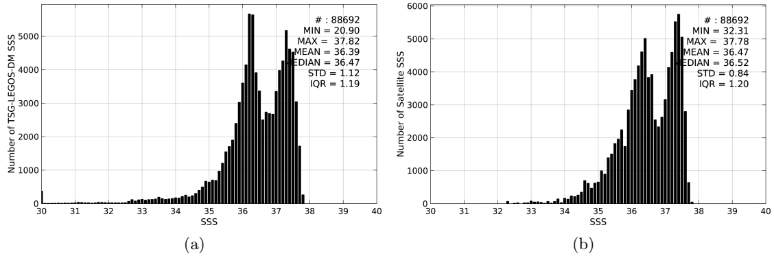
Figure 2: Histograms of SSS from TSG-LEGOS-DM (a) and Aquarius-L4-IPRC-V4-WEEKLY (b) considering all match-up pairs per bins of 0.1 over the Amazon and Orinoco river plumes Pi-MEP region and for the full satellite product period.
