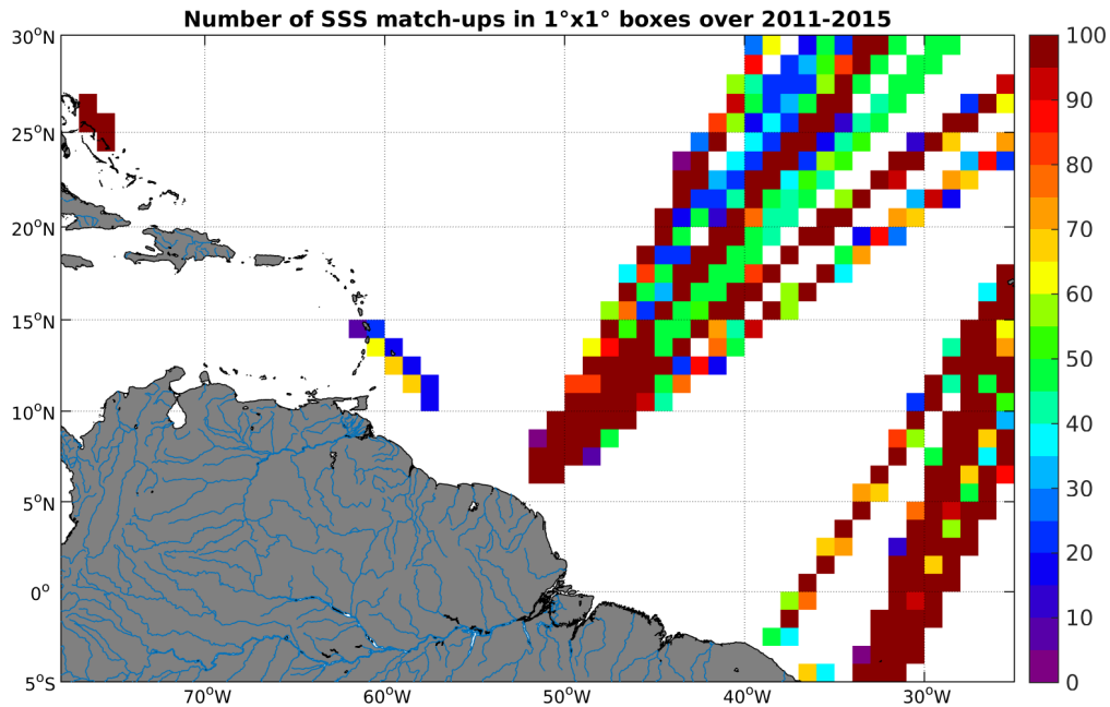
Figure 4: Number of SSS match-ups between TSG-LEGOS-DM SSS and the Aquarius-L4-IPRC-V4-WEEKLY SSS product for the Amazon and Orinoco river plumes Pi-MEP region over 1^\circ \times 1^\circ boxes and for the full satellite product period.
