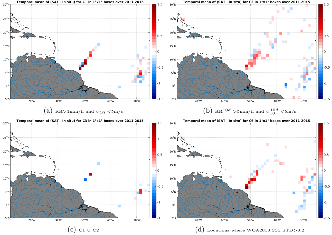
Figure 12: Temporal mean gridded over spatial boxes of size 1^\circ \times 1^\circ of \Delta SSS (Aquarius-L4-IPRC-V4-WEEKLY - TSG-LEGOS-DM) for 4 different subdatasets corresponding to: RR > 1mm/h and U_{10} < 5 m/s (a), RR^{10d} > 5 mm/h and U_{10}^{10d} < 5 m/s (b), C1 U C2 (c), Locations where WOA2013 SSS STD > 0.2 (d).
