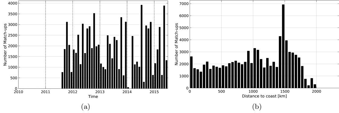
Figure 1: Number of match-ups between TSG-LEGOS-DM and Aquarius-L4-IPRC-V4-WEEKLY SSS as a function of time (a) and as function of the distance to coast (b) over the Amazon and Orinoco river plumes Pi-MEP region and for the full satellite product period.
