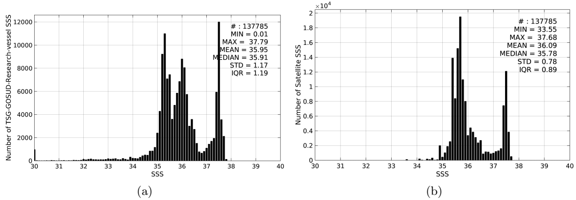
Figure 2: Histograms of SSS from TSG-GOSUD-Research-vessel (a) and Aquarius-L4-IPRC-V4-WEEKLY (b) considering all match-up pairs per bins of 0.1 over the Amazon and Orinoco river plumes Pi-MEP region and for the full satellite product period.
