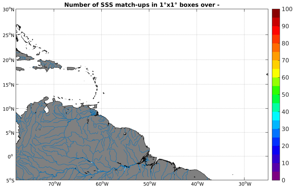
Figure 4: Number of SSS match-ups between Sea mammals SSS and the Aquarius-L4-IPRC-V4-WEEKLY SSS product for the Amazon and Orinoco river plumes Pi-MEP region over 1^\circ \times 1^\circ boxes and for the full satellite product period.
