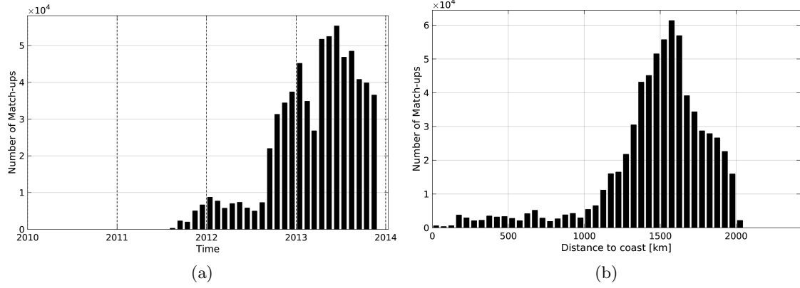
Figure 1: Number of match-ups between Surface drifters and Aquarius-L4-IPRC-V4-WEEKLY SSS as a function of time (a) and as function of the distance to coast (b) over the Amazon and Orinoco river plumes Pi-MEP region and for the full satellite product period.
