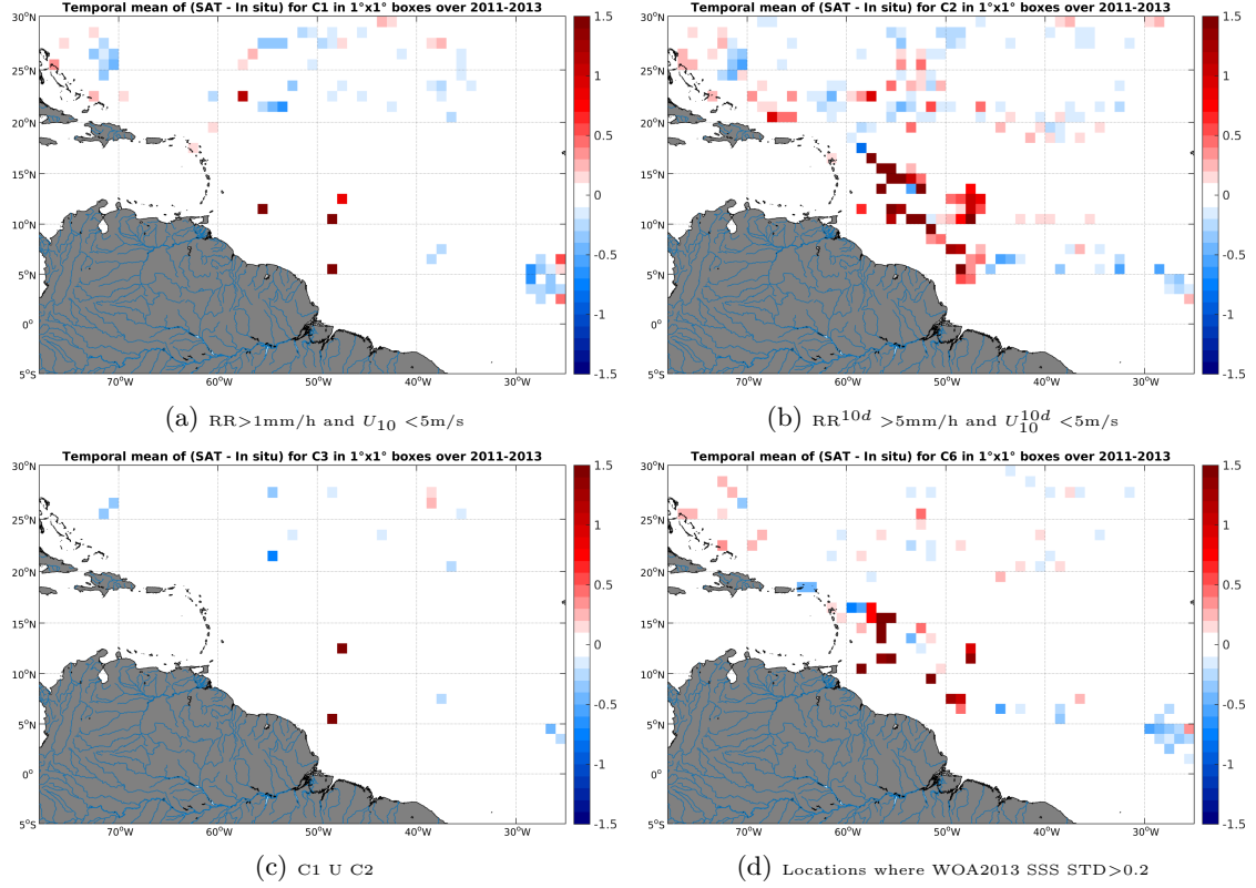
Figure 11: Temporal mean gridded over spatial boxes of size 1^\circ \times 1^\circ of \Delta SSS (Aquarius-L4-IPRC-V4-WEEKLY - Surface drifters) for 4 different subdatasets corresponding to: RR > 1 mm/h and U_{10} < 5 m/s (a), RR 10d > 5 mm/h and U_{10}^{10d} < 5 m/s (b), C1 U C2 (c), Locations where WOA2013 SSS STD > 0.2 (d).
