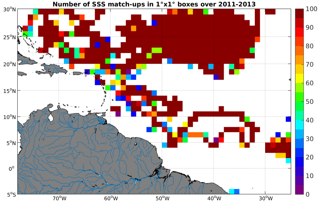
Figure 3: Number of SSS match-ups between Surface drifters SSS and the Aquarius-L4-IPRC-V4-WEEKLY SSS product for the Amazon and Orinoco river plumes Pi-MEP region over 1^\circ \times 1^\circ boxes and for the full satellite product period.
