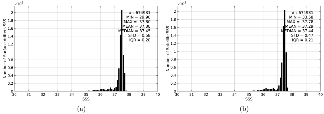
Figure 2: Histograms of SSS from Surface drifters (a) and Aquarius-L4-IPRC-V4-WEEKLY (b) considering all match-up pairs per bins of 0.1 over the Amazon and Orinoco river plumes Pi-MEP region and for the full satellite product period.
