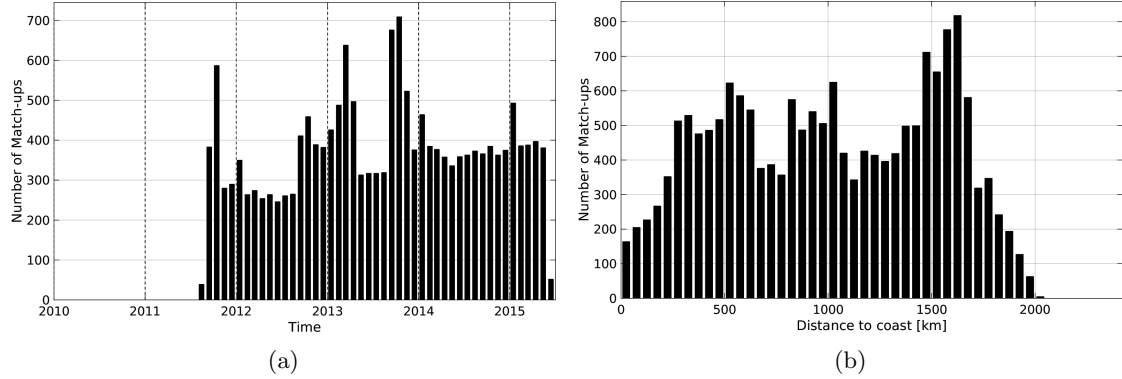
Figure 1: Number of match-ups between Argo and Aquarius-L4-IPRC-V4-WEEKLY SSS as a function of time (a) and as function of the distance to coast (b) over the Amazon and Orinoco river plumes Pi-MEP region and for the full satellite product period.
