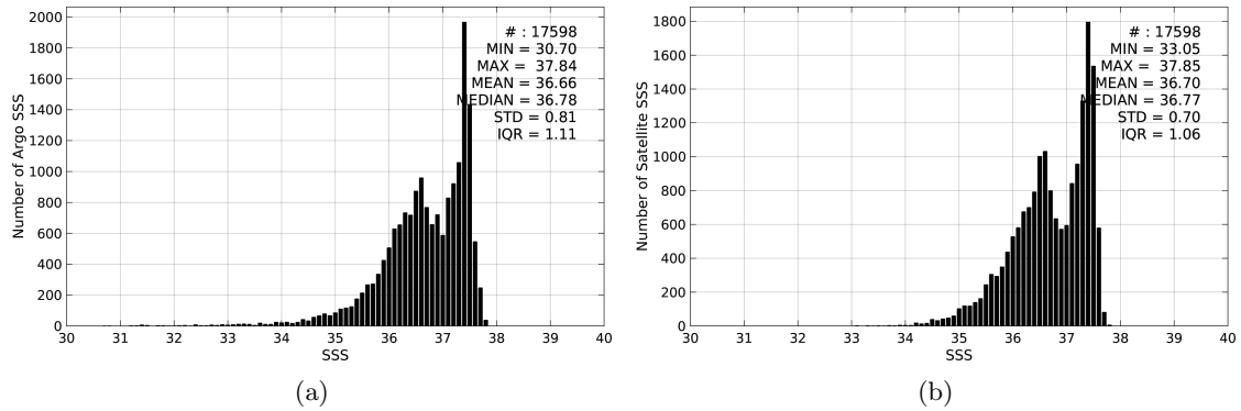
Figure 2: Histograms of SSS from Argo (a) and Aquarius-L4-IPRC-V4-WEEKLY (b) considering all match-up pairs per bins of 0.1 over the Amazon and Orinoco river plumes Pi-MEP region and for the full satellite product period.
