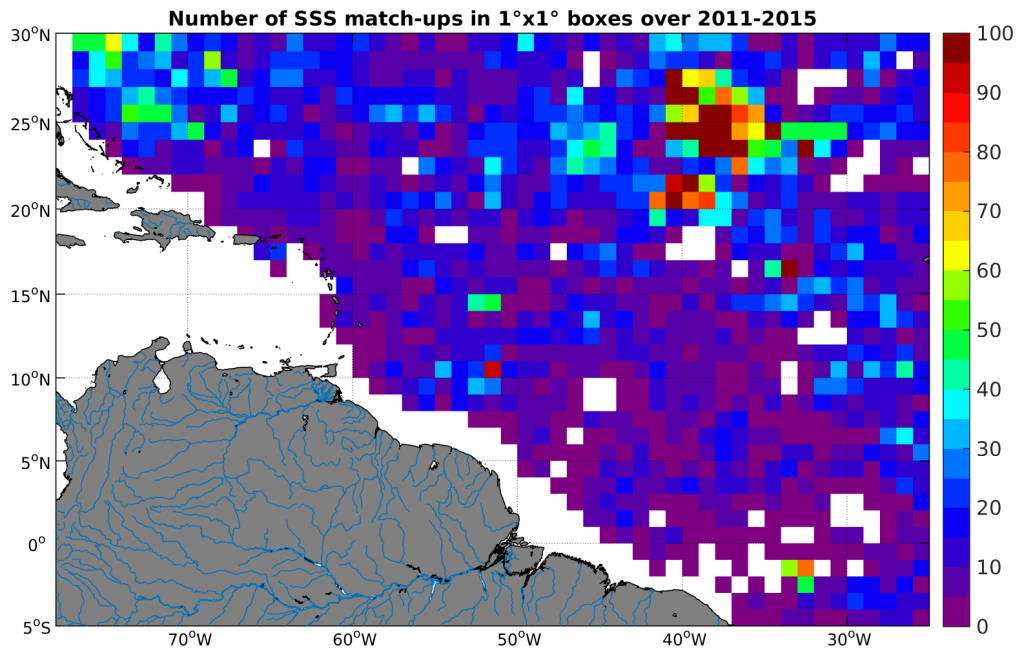
Figure 4: Number of SSS match-ups between Argo SSS and the Aquarius-L4-IPRC-V4-WEEKLY SSS product for the Amazon and Orinoco river plumes Pi-MEP region over 1^\circ \times 1^\circ boxes and for the full satellite product period.
