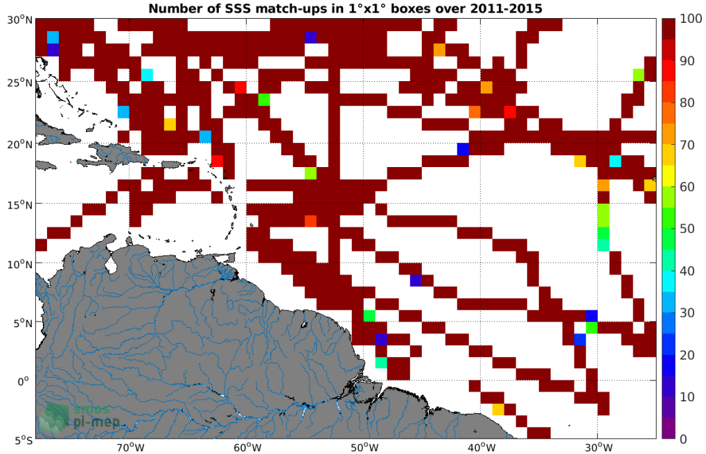
Figure 4: Number of SSS match-ups between TSG (SAMOS) SSS and the Aquarius SSS L3 CAP v5 - 7-Day running (JPL) SSS product for the Amazon and Orinoco river plumes Pi-MEP region over 1^\circ \times 1^\circ boxes and for the full satellite product period.
