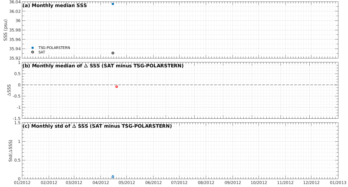
Figure 7: Time series of the monthly median SSS (top), median of \Delta\text{SSS} (Satellite - TSG-POLARSTERN) and Std of \Delta\text{SSS} (Satellite - TSG-POLARSTERN) over the Amazon and Orinoco river plumes Pi-MEP region considering all match-ups collected by the Pi-MEP.
