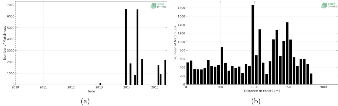
Figure 1: Number of match-ups between TSG (GOSUD-Sailing-ship) and Aquarius SSS L3 CAP v5 - 7-Day running (JPL) SSS as a function of time (a) and as function of the distance to coast (b) over the Amazon and Orinoco river plumes Pi-MEP region and for the full satellite product period.
