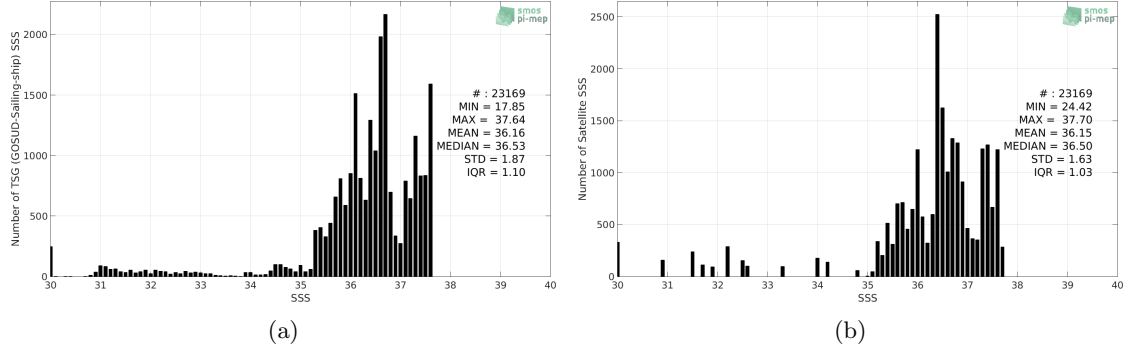
Figure 2: Histograms of SSS from TSG (GOSUD-Sailing-ship) (a) and Aquarius SSS L3 CAP v5 - 7-Day running (JPL) (b) considering all match-up pairs per bins of 0.1 over the Amazon and Orinoco river plumes Pi-MEP region and for the full satellite product period.
