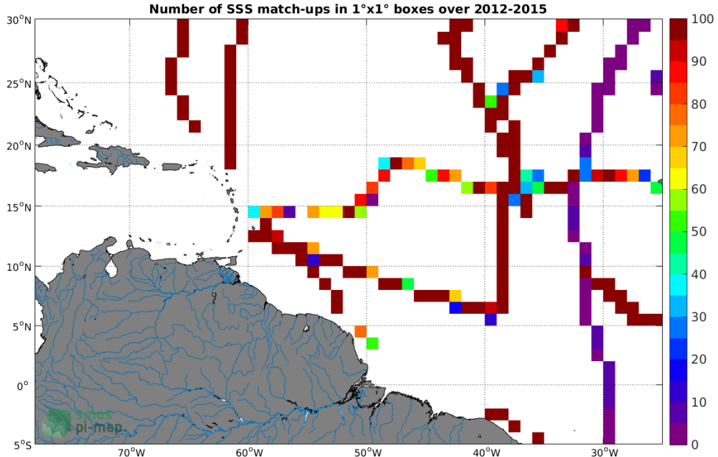
Figure 4: Number of SSS match-ups between TSG (GOSUD-Sailing-ship) SSS and the Aquarius SSS L3 CAP v5 - 7-Day running (JPL) SSS product for the Amazon and Orinoco river plumes Pi-MEP region over 1^\circ \times 1^\circ boxes and for the full satellite product period.
