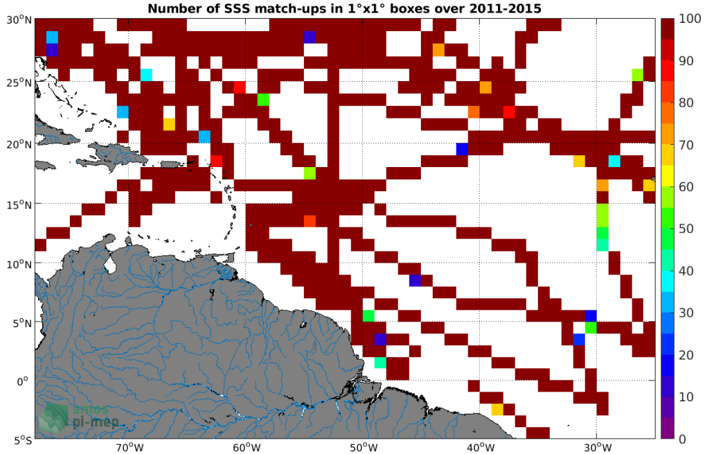
Figure 4: Number of SSS match-ups between TSG (SAMOS) SSS and the Aquarius SSS L3 CAP v5 - Monthly (JPL) SSS product for the Amazon and Orinoco river plumes Pi-MEP region over 1^\circ \times 1^\circ boxes and for the full satellite product period.
