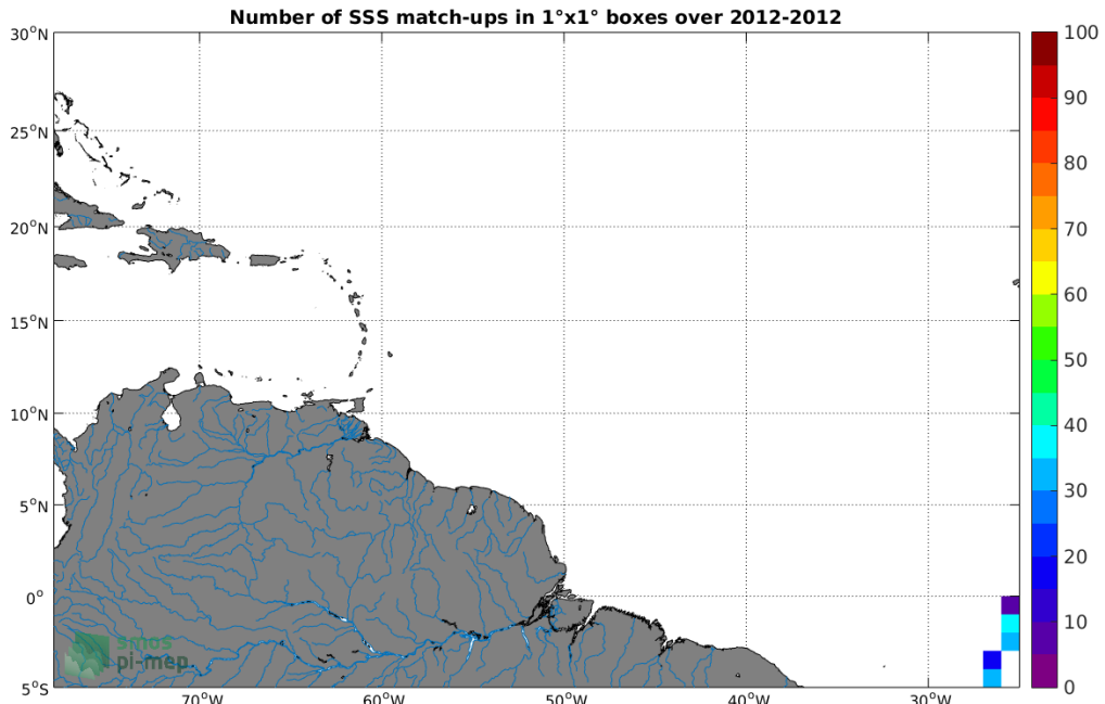
Figure 4: Number of SSS match-ups between TSG-POLARSTERN SSS and the Aquarius-L3-JPL-V5-MONTHLY SSS product for the Amazon and Orinoco river plumes Pi-MEP region over 1°x1° boxes and for the full satellite product period.
