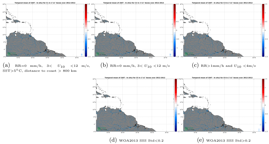
Figure 12: Temporal mean gridded over spatial boxes of size 1^\circ \times 1^\circ of \Delta SSS (Aquarius-L3-JPL-V5-MONTHLY - TSG-POLARSTERN) for 5 different subdatasets corresponding to:RR=0 mm/h, 3 < U_{10} < 12 m/s, SST >5^\circ C, distance to coast > 800 km (a), RR=0 mm/h, 3 < U_{10} < 12 m/s (b), RR >1 mm/h and U_{10} < 4 m/s (c), WOA2013 SSS Std <0.2 (d), WOA2013 SSS Std >0.2 (e).
