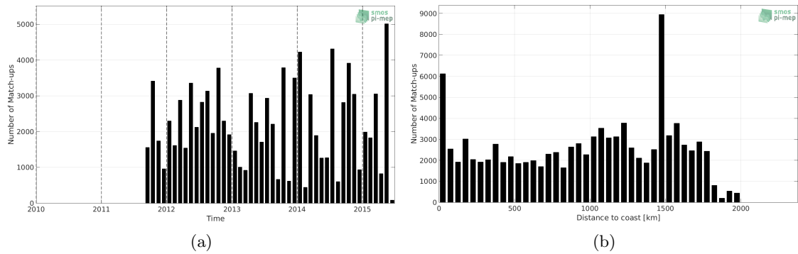
Figure 1: Number of match-ups between TSG-LEGOS-DM and Aquarius-L3-JPL-V5-MONTHLY SSS as a function of time (a) and as function of the distance to coast (b) over the Amazon and Orinoco river plumes Pi-MEP region and for the full satellite product period.
