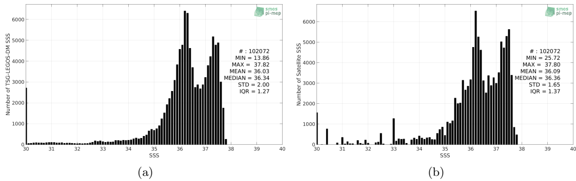
Figure 2: Histograms of SSS from TSG-LEGOS-DM (a) and Aquarius-L3-JPL-V5-MONTHLY (b) considering all match-up pairs per bins of 0.1 over the Amazon and Orinoco river plumes Pi-MEP region and for the full satellite product period.
