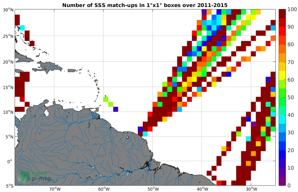
Figure 4: Number of SSS match-ups between TSG-LEGOS-DM SSS and the Aquarius-L3-JPL-V5-MONTHLY SSS product for the Amazon and Orinoco river plumes Pi-MEP region over 1^\circ \times 1^\circ boxes and for the full satellite product period.
