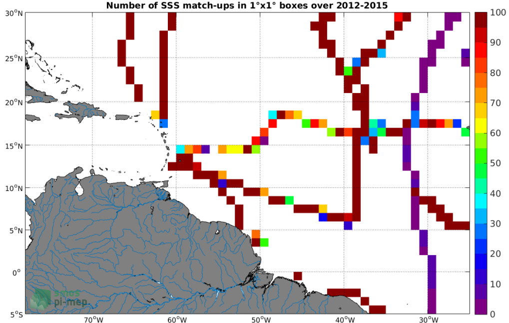
Figure 4: Number of SSS match-ups between TSG (GOSUD-Sailing-ship) SSS and the Aquarius SSS L3 CAP v5 - Monthly (JPL) SSS product for the Amazon and Orinoco river plumes Pi-MEP region over 1^\circ \times 1^\circ boxes and for the full satellite product period.
