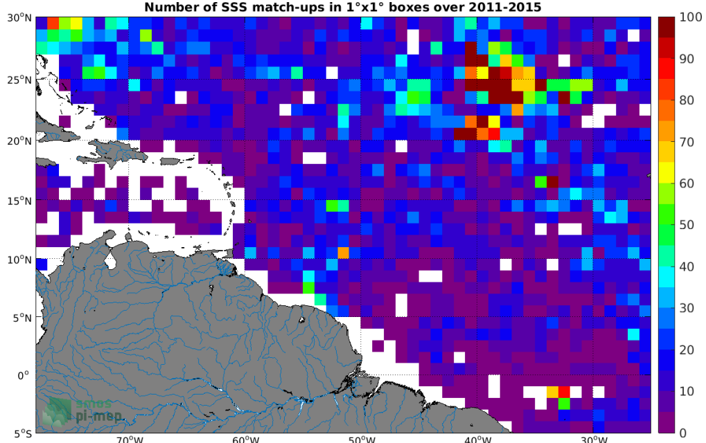
Figure 4: Number of SSS match-ups between Argo SSS and the Aquarius SSS L3 CAP v5 - Monthly (JPL) SSS product for the Amazon and Orinoco river plumes Pi-MEP region over 1°x1° boxes and for the full satellite product period.
