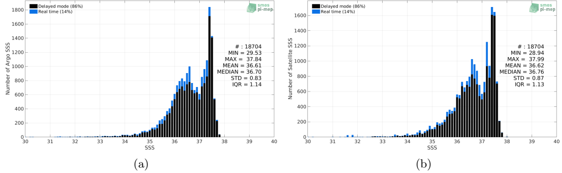
Figure 2: Histograms of SSS from Argo (a) and Aquarius SSS L3 CAP v5 - Monthly (JPL) (b) considering all match-up pairs per bins of 0.1 over the Amazon and Orinoco river plumes Pi-MEP region and for the full satellite product period.
