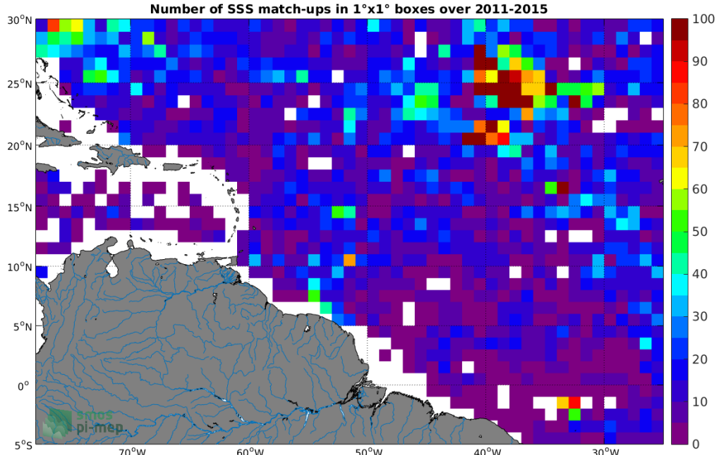
Figure 4: Number of SSS match-ups between Argo SSS and the Aquarius-L3-JPL-V5-MONTHLY SSS product for the Amazon and Orinoco river plumes Pi-MEP region over 1^\circ \times 1^\circ boxes and for the full satellite product period.
