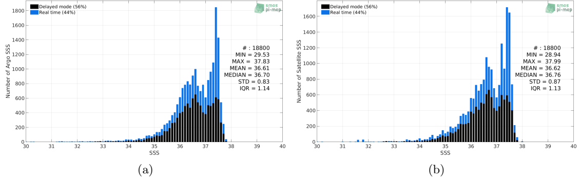
Figure 2: Histograms of SSS from Argo (a) and Aquarius-L3-JPL-V5-MONTHLY (b) considering all match-up pairs per bins of 0.1 over the Amazon and Orinoco river plumes Pi-MEP region and for the full satellite product period.
