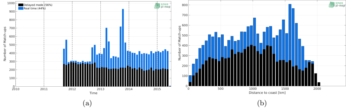
Figure 1: Number of match-ups between Argo and Aquarius-L3-JPL-V5-MONTHLY SSS as a function of time (a) and as function of the distance to coast (b) over the Amazon and Orinoco river plumes Pi-MEP region and for the full satellite product period.
