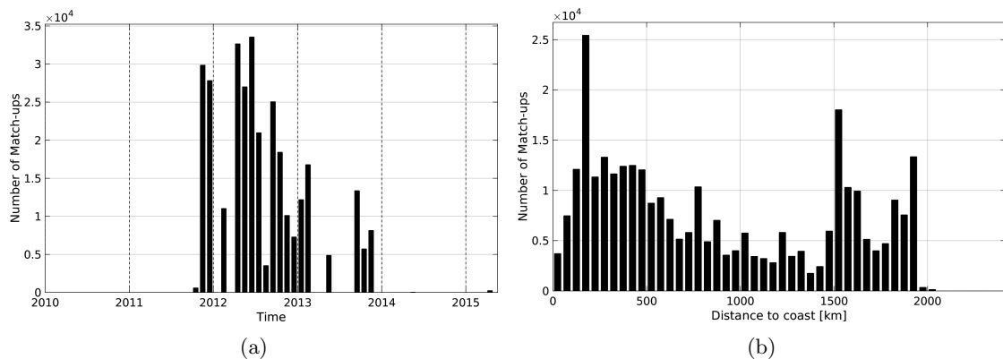
Figure 1: Number of match-ups between TSG-SAMOS and Aquarius-L3-JPL-V4-7DAY-RUNNING SSS as a function of time (a) and as function of the distance to coast (b) over the Amazon and Orinoco river plumes Pi-MEP region and for the full satellite product period.
