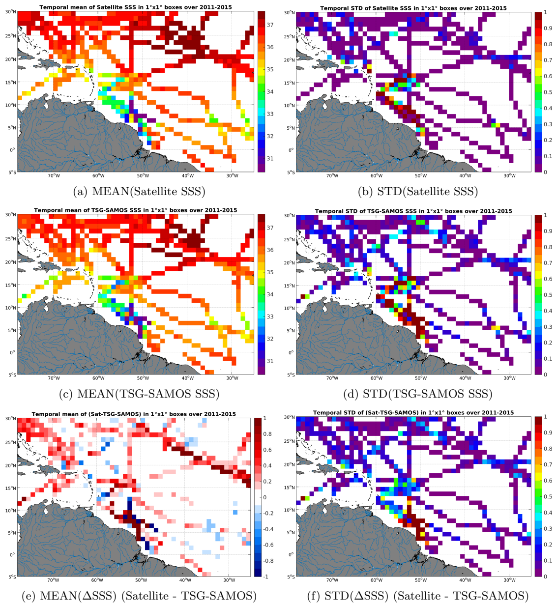
Figure 6: Temporal mean (left) and STD (right) of SSS from Aquarius-L3-JPL-V4-7DAY-RUNNING (top), TSG-SAMOS (middle), and of \Delta SSS (Satellite - TSG-SAMOS). Only match-up pairs are used to generate these maps.
