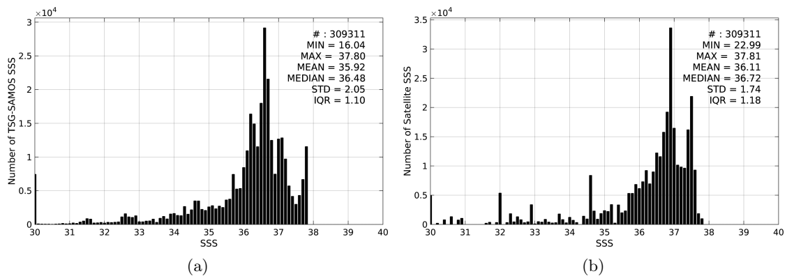
Figure 2: Histograms of SSS from TSG-SAMOS (a) and Aquarius-L3-JPL-V4-7DAY-RUNNING (b) considering all match-up pairs per bins of 0.1 over the Amazon and Orinoco river plumes Pi-MEP region and for the full satellite product period.
