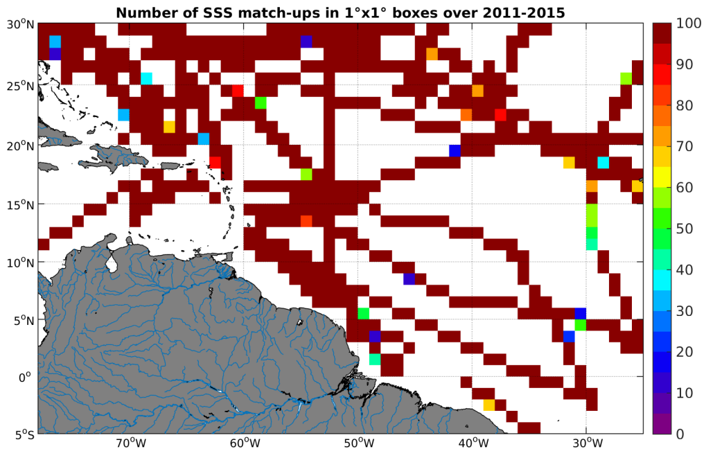
Figure 4: Number of SSS match-ups between TSG-SAMOS SSS and the Aquarius-L3-JPL-V4-7DAY-RUNNING SSS product for the Amazon and Orinoco river plumes Pi-MEP region over 1^\circ \times 1^\circ boxes and for the full satellite product period.
