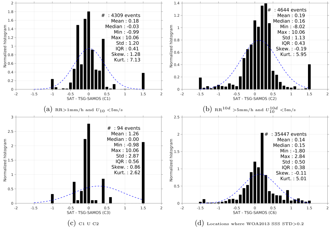
Figure 13: Normalized histogram of \Delta\text{SSS} (Aquarius-L3-JPL-V4-7DAY-RUNNING - TSG-SAMOS) for 6 different subdatasets corresponding to: RR>1mm/h and U_{10} < 5\text{m/s} (a), \text{RR}^{10d} > 5\text{mm/h} and U_{10}^{10d} < 5\text{m/s} (b), C1 U C2 (c), Locations where WOA2013 SSS STD>0.2 (d).
