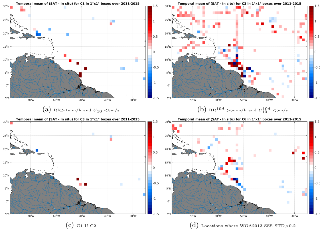
Figure 12: Temporal mean gridded over spatial boxes of size 1^\circ \times 1^\circ of \Delta SSS (Aquarius-L3-JPL-V4-7DAY-RUNNING - TSG-SAMOS) for 4 different subdatasets corresponding to: RR > 1\text{mm/h} and U_{10} < 5\text{m/s} (a), RR^{10d} > 5\text{mm/h} and U_{10}^{10d} < 5\text{m/s} (b), C1 U C2 (c), Locations where WOA2013 SSS STD > 0.2 (d).
