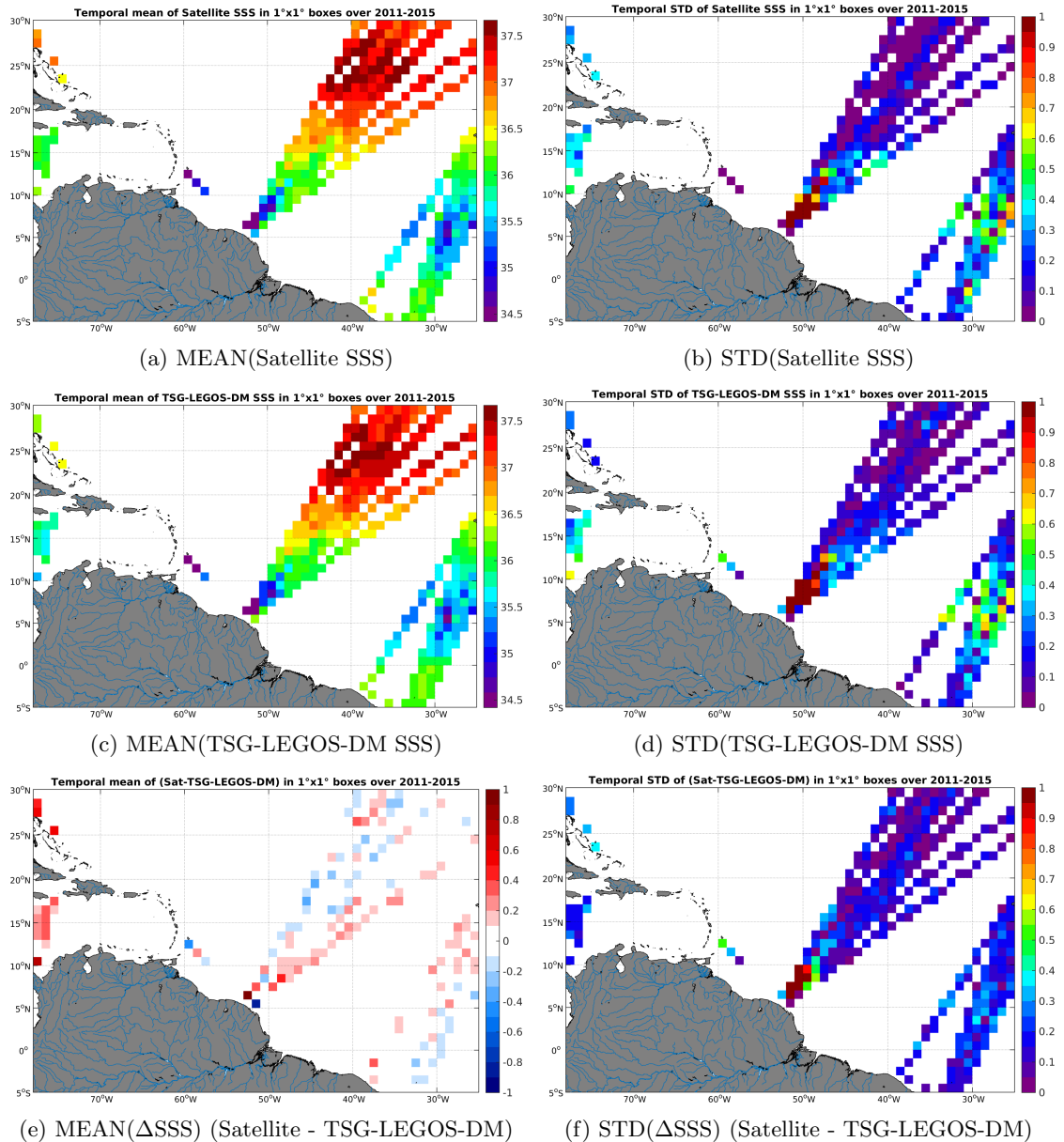
Figure 6: Temporal mean (left) and STD (right) of SSS from Aquarius-L3-JPL-V4-7DAY-RUNNING (top), TSG-LEGOS-DM (middle), and of \Delta SSS (Satellite - TSG-LEGOS-DM). Only match-up pairs are used to generate these maps.
