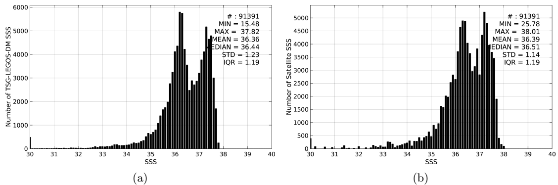
Figure 2: Histograms of SSS from TSG-LEGOS-DM (a) and Aquarius-L3-JPL-V4-7DAY-RUNNING (b) considering all match-up pairs per bins of 0.1 over the Amazon and Orinoco river plumes Pi-MEP region and for the full satellite product period.
