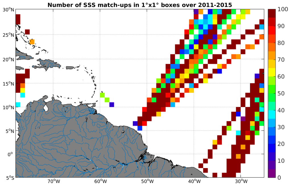
Figure 4: Number of SSS match-ups between TSG-LEGOS-DM SSS and the Aquarius-L3-JPL-V4-7DAY-RUNNING SSS product for the Amazon and Orinoco river plumes Pi-MEP region over 1^\circ \times 1^\circ boxes and for the full satellite product period.
