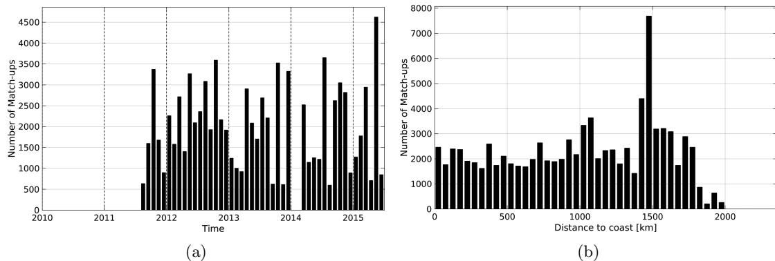
Figure 1: Number of match-ups between TSG-LEGOS-DM and Aquarius-L3-JPL-V4-7DAY-RUNNING SSS as a function of time (a) and as function of the distance to coast (b) over the Amazon and Orinoco river plumes Pi-MEP region and for the full satellite product period.
