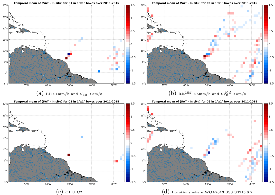
Figure 12: Temporal mean gridded over spatial boxes of size 1^\circ \times 1^\circ of \Delta SSS (Aquarius-L3-JPL-V4-7DAY-RUNNING - TSG-LEGOS-DM) for 4 different subdatasets corresponding to: RR > 1\text{mm/h} and U_{10} < 5\text{m/s} (a), RR^{10d} > 5\text{mm/h} and U_{10}^{10d} < 5\text{m/s} (b), C1 U C2 (c), Locations where WOA2013 SSS STD > 0.2 (d).
