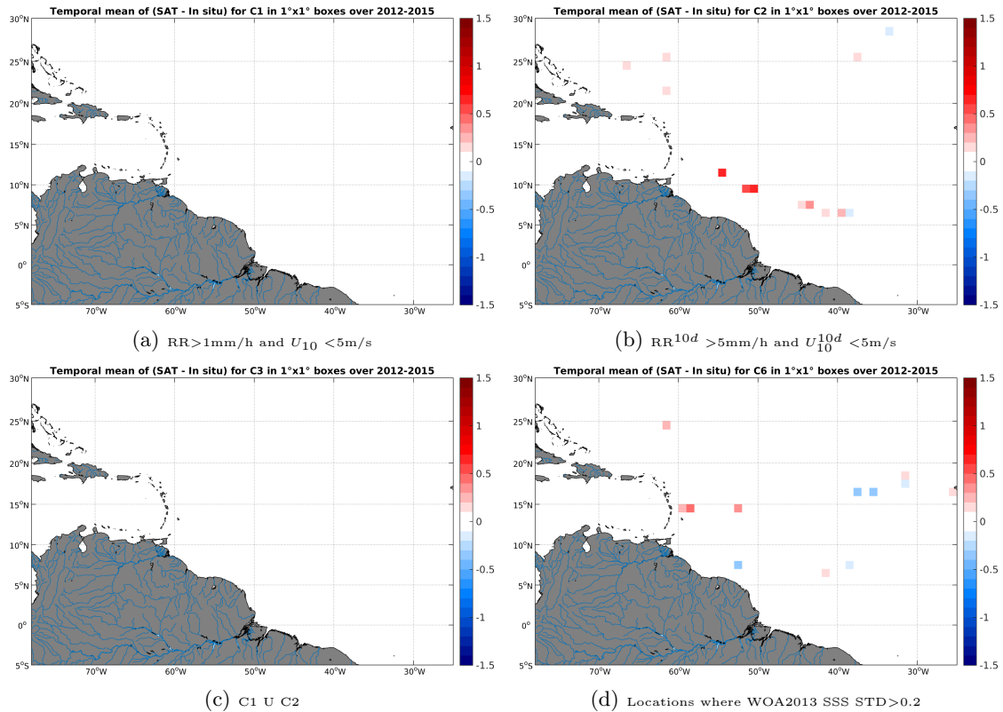
Figure 12: Temporal mean gridded over spatial boxes of size 1°x1° of \Delta SSS (Aquarius-L3-JPL-V4-7DAY-RUNNING - TSG-GOSUD-Sailing-ship) for 4 different subdatasets corresponding to:RR>1mm/h and U_{10} < 5\text{m/s} (a), RR^{10d} > 5\text{mm/h} and U_{10}^{10d} < 5\text{m/s} (b), C1 U C2 (c),Locations where WOA2013 SSS STD>0.2 (d).
