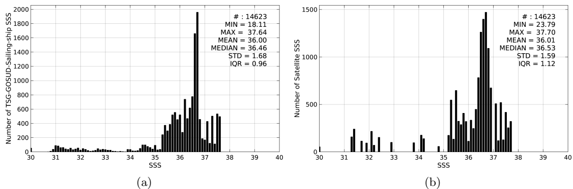
Figure 2: Histograms of SSS from TSG-GOSUD-Sailing-ship (a) and Aquarius-L3-JPL-V4-7DAY-RUNNING (b) considering all match-up pairs per bins of 0.1 over the Amazon and Orinoco river plumes Pi-MEP region and for the full satellite product period.
