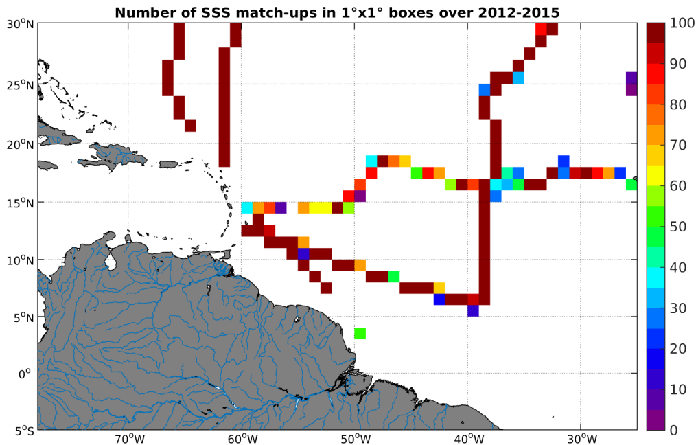
Figure 4: Number of SSS match-ups between TSG-GOSUD-Sailing-ship SSS and the Aquarius-L3-JPL-V4-7DAY-RUNNING SSS product for the Amazon and Orinoco river plumes Pi-MEP region over 1°x1° boxes and for the full satellite product period.
