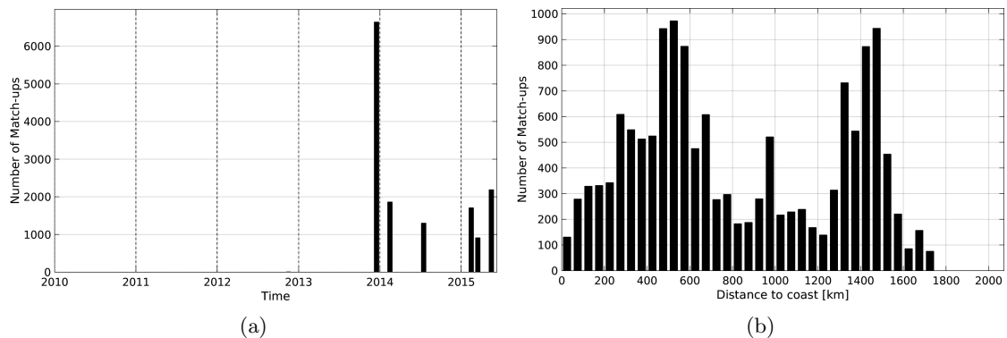
Figure 1: Number of match-ups between TSG-GOSUD-Sailing-ship and Aquarius-L3-JPL-V4-7DAY-RUNNING SSS as a function of time (a) and as function of the distance to coast (b) over the Amazon and Orinoco river plumes Pi-MEP region and for the full satellite product period.
