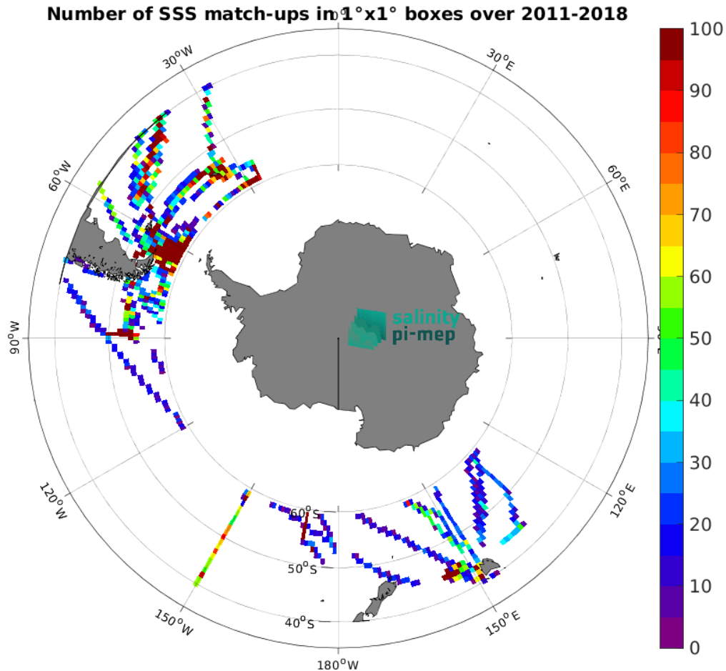
Figure 4: Number of SSS match-ups between TSG (SAMOS) SSS and the SMOS and SMAP SSS L4 OI v1 - 7 Days (LOPS) SSS product for the Roaring Forties and Furious Fifties Pi-MEP region over 1^\circ \times 1^\circ boxes and for the full satellite product period.
