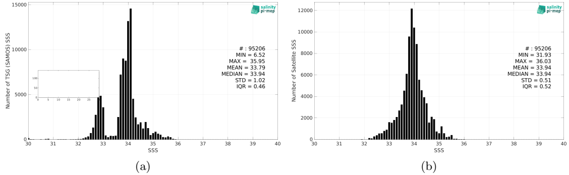
Figure 2: Histograms of SSS from TSG (SAMOS) (a) and SMOS and SMAP SSS L4 OI v1 - 7 Days (LOPS) (b) considering all match-up pairs per bins of 0.1 over the Roaring Forties and Furious Fifties Pi-MEP region and for the full satellite product period.
