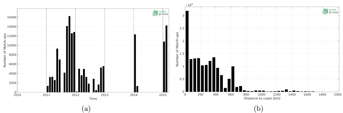
Figure 1: Number of match-ups between TSG (SAMOS) and SMOS and SMAP SSS L4 OI v1 - 7 Days (LOPS) SSS as a function of time (a) and as function of the distance to coast (b) over the Roaring Forties and Furious Fifties Pi-MEP region and for the full satellite product period.
