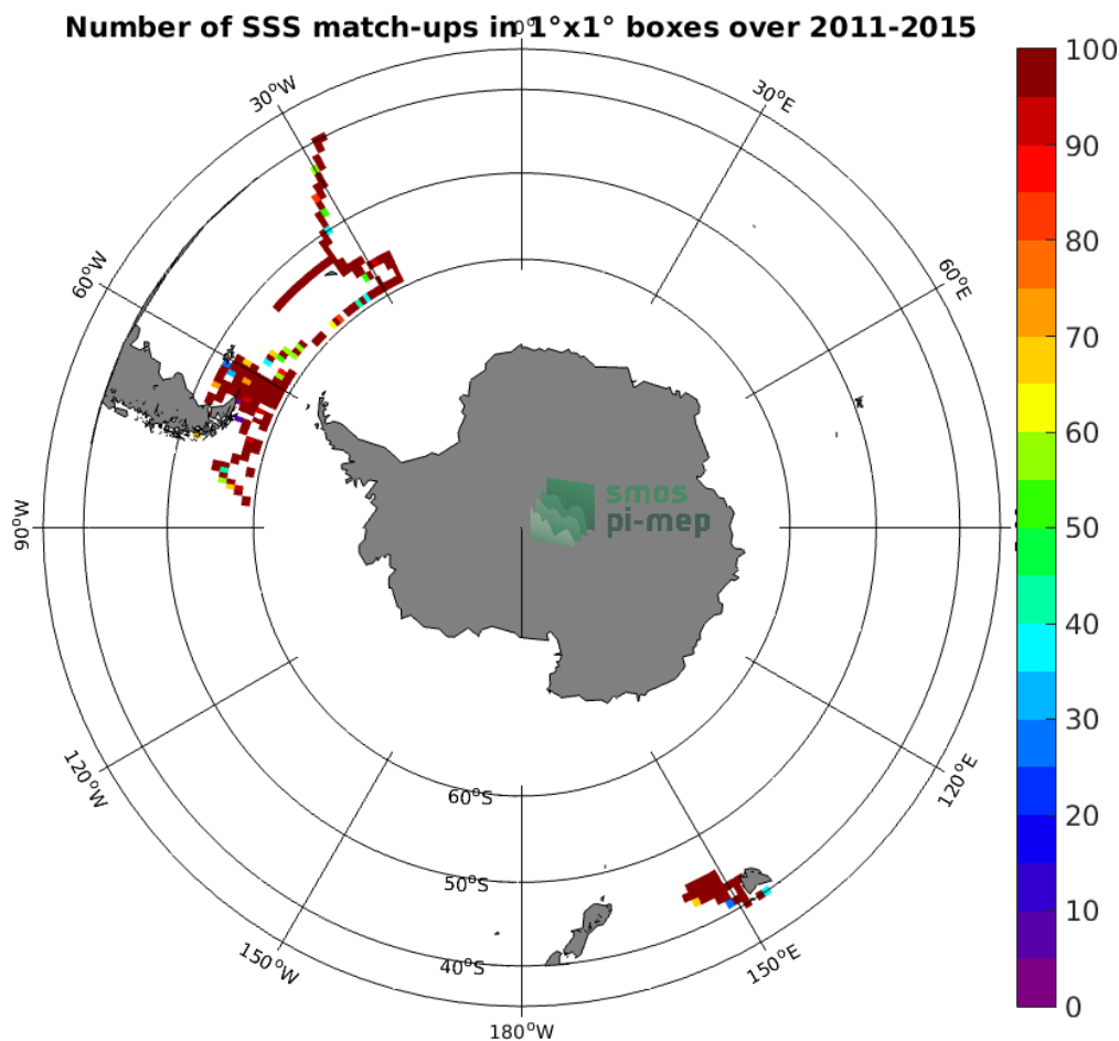
Figure 4: Number of SSS match-ups between TSG (SAMOS) SSS and the SMOS and SMAP SSS L4 OI v1 - 7 Days (LOPS) SSS product for the Roaring Forties and Furious Fifties Pi-MEP region over 1^\circ \times 1^\circ boxes and for the full satellite product period.
