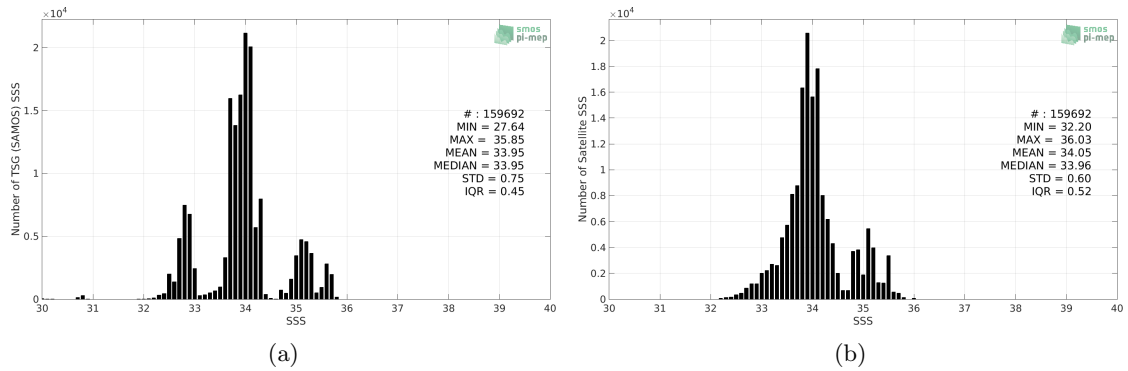
Figure 2: Histograms of SSS from TSG (SAMOS) (a) and SMOS and SMAP SSS L4 OI v1 - 7 Days (LOPS) (b) considering all match-up pairs per bins of 0.1 over the Roaring Forties and Furious Fifties Pi-MEP region and for the full satellite product period.
