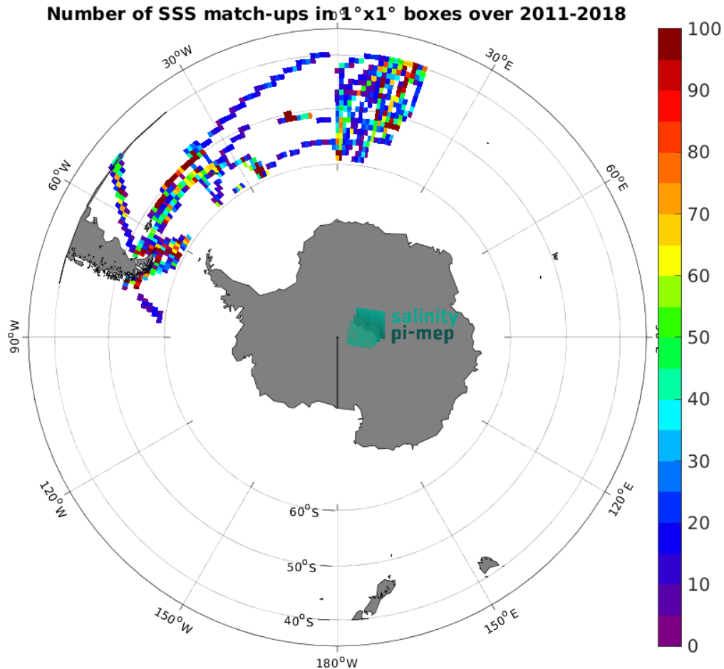
Figure 4: Number of SSS match-ups between TSG (Polarstern) SSS and the SMOS and SMAP SSS L4 OI v1 - 7 Days (LOPS) SSS product for the Roaring Forties and Furious Fifties Pi-MEP region over 1^\circ \times 1^\circ boxes and for the full satellite product period.
