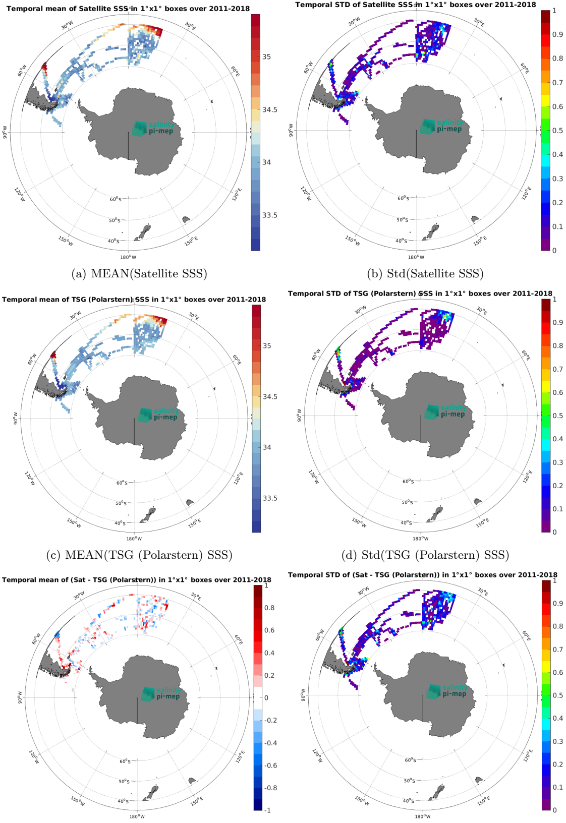
(e) MEAN( \Delta SSS) (Satellite - TSG (Polarstern)) 16 (f) Std( \Delta SSS) (Satellite - TSG (Polarstern)) Figure 6: Temporal mean (left) and Std (right) of SSS from SMOS and SMAP SSS L4 OI v1 - 7 Days (LOPS) (top), TSG (Polarstern) (middle), and of \Delta SSS (Satellite - TSG (Polarstern)). Only match-up pairs are used to generate these maps.
