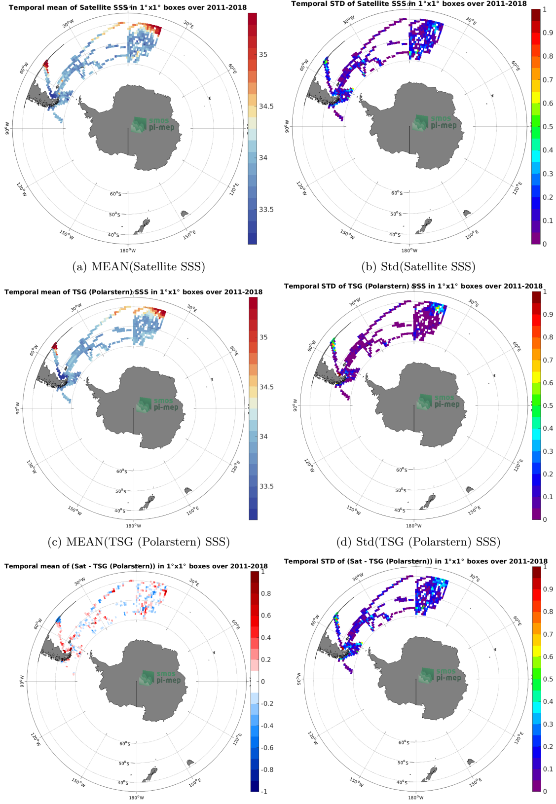
Figure 6: Temporal mean (left) and Std (right) of SSS from SMOS and SMAP SSS L4 OI v1 - 7 Days (LOPS) (top), TSG (Polarstern) (middle), and of \Delta SSS (Satellite - TSG (Polarstern)). Only match-up pairs are used to generate these maps.
