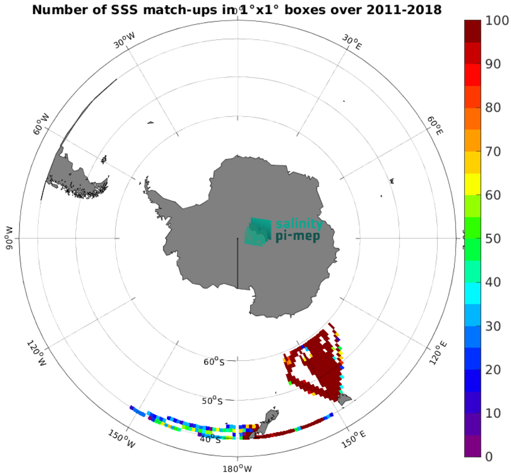
Figure 4: Number of SSS match-ups between TSG (LEGOS-DM) SSS and the SMOS and SMAP SSS L4 OI v1 - 7 Days (LOPS) SSS product for the Roaring Forties and Furious Fifties Pi-MEP region over 1^\circ \times 1^\circ boxes and for the full satellite product period.
