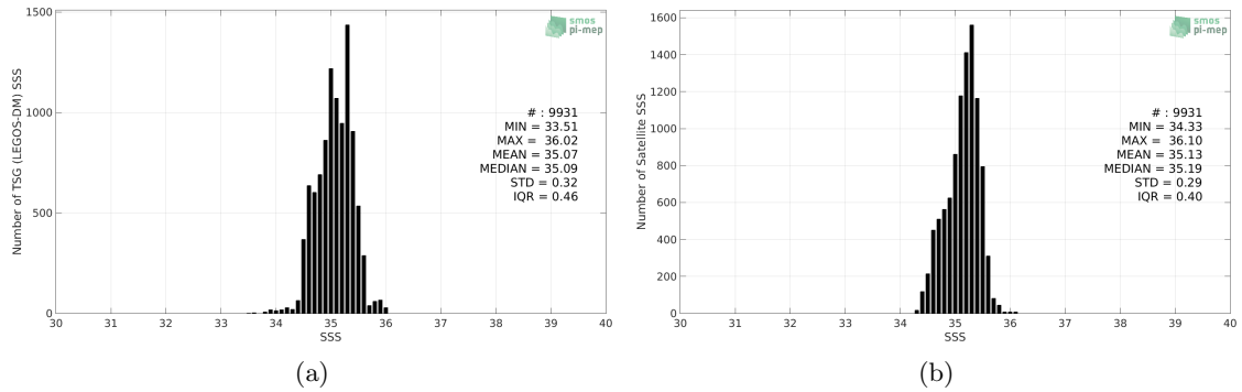
Figure 2: Histograms of SSS from TSG (LEGOS-DM) (a) and SMOS and SMAP SSS L4 OI v1 - 7 Days (LOPS) (b) considering all match-up pairs per bins of 0.1 over the Roaring Forties and Furious Fifties Pi-MEP region and for the full satellite product period.
