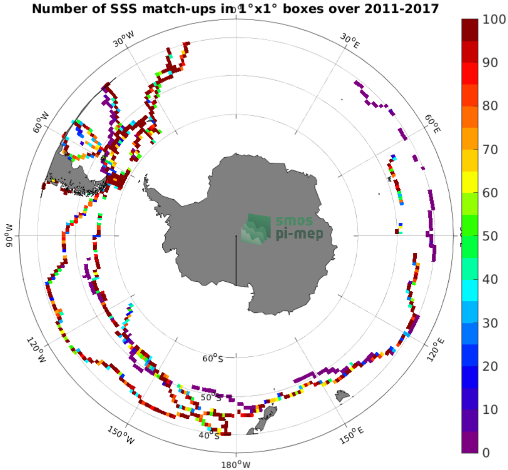
Figure 4: Number of SSS match-ups between TSG (GOSUD-Sailing-ship) SSS and the SMOS and SMAP SSS L4 OI v1 - 7 Days (LOPS) SSS product for the Roaring Forties and Furious Fifties Pi-MEP region over 1^\circ \times 1^\circ boxes and for the full satellite product period.
