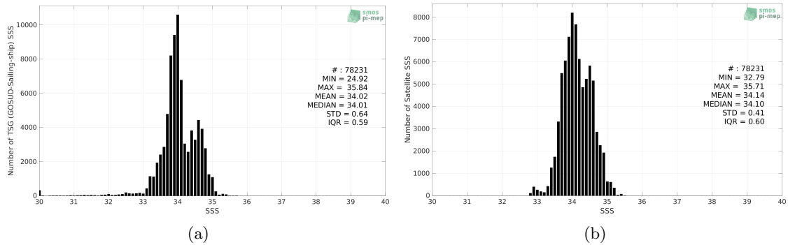
Figure 2: Histograms of SSS from TSG (GOSUD-Sailing-ship) (a) and SMOS and SMAP SSS L4 OI v1 - 7 Days (LOPS) (b) considering all match-up pairs per bins of 0.1 over the Roaring Forties and Furious Fifties Pi-MEP region and for the full satellite product period.
