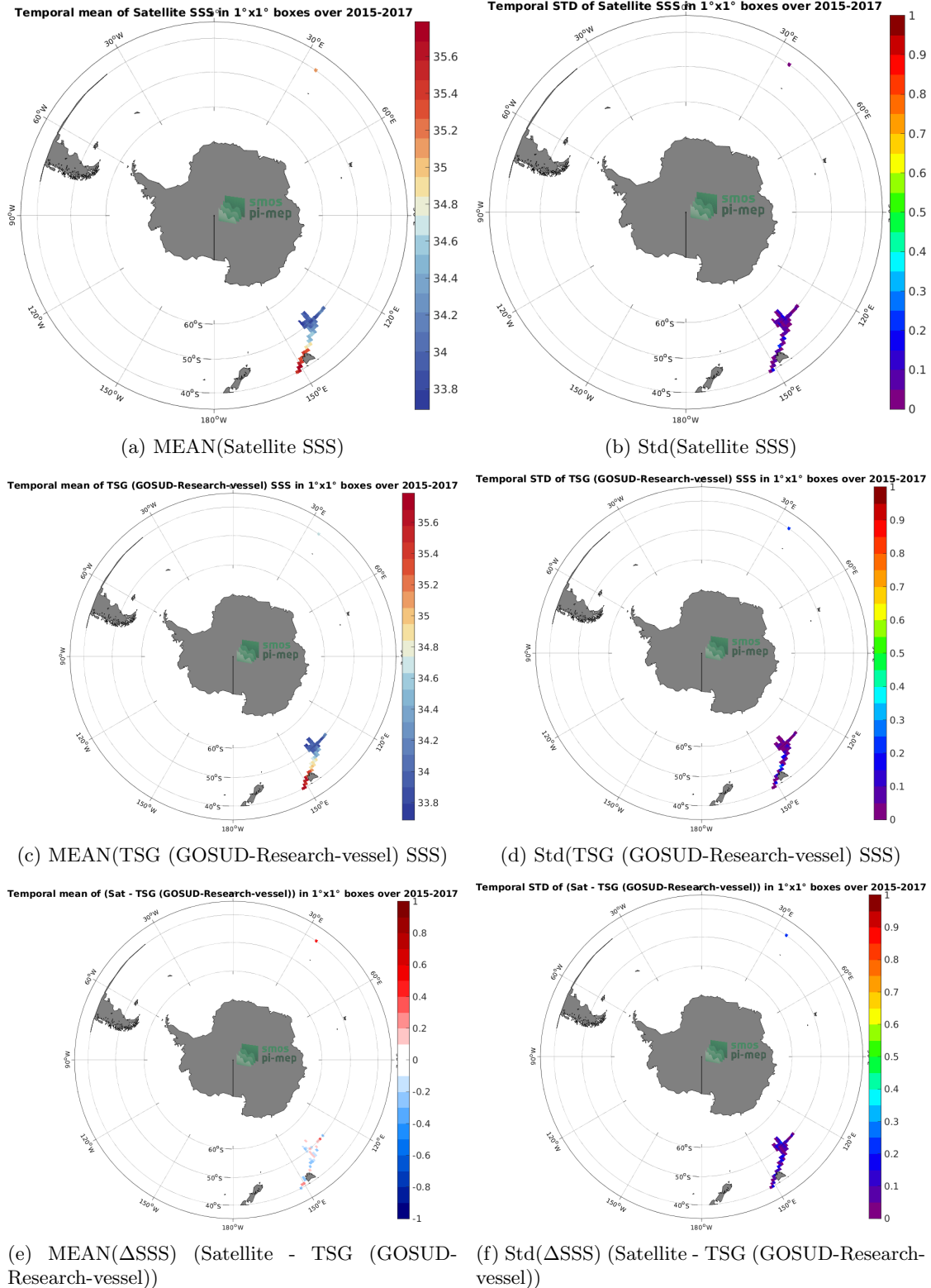
Figure 6: Temporal mean (left) and Std (right) of SSS from SMOS and SMAP SSS L4 OI v1 - 7 Days (LOPS) (top), TSG (GOSUD-Research-vessel) (middle), and of \Delta SSS (Satellite - TSG (GOSUD-Research-vessel)). Only match-up pairs are used to generate these maps.
