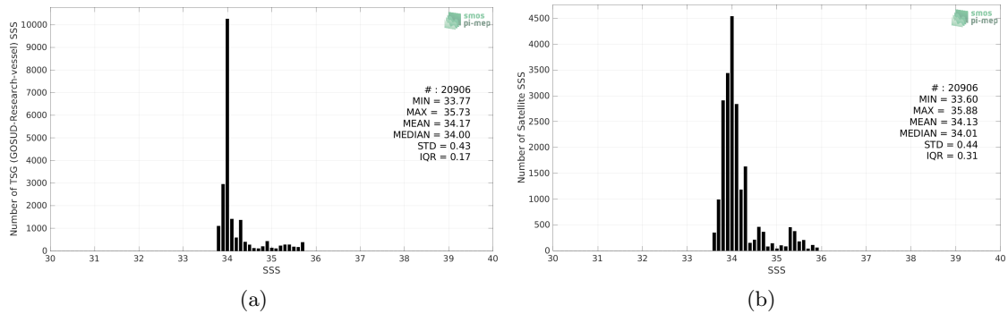
Figure 2: Histograms of SSS from TSG (GOSUD-Research-vessel) (a) and SMOS and SMAP SSS L4 OI v1 - 7 Days (LOPS) (b) considering all match-up pairs per bins of 0.1 over the Roaring Forties and Furious Fifties Pi-MEP region and for the full satellite product period.
