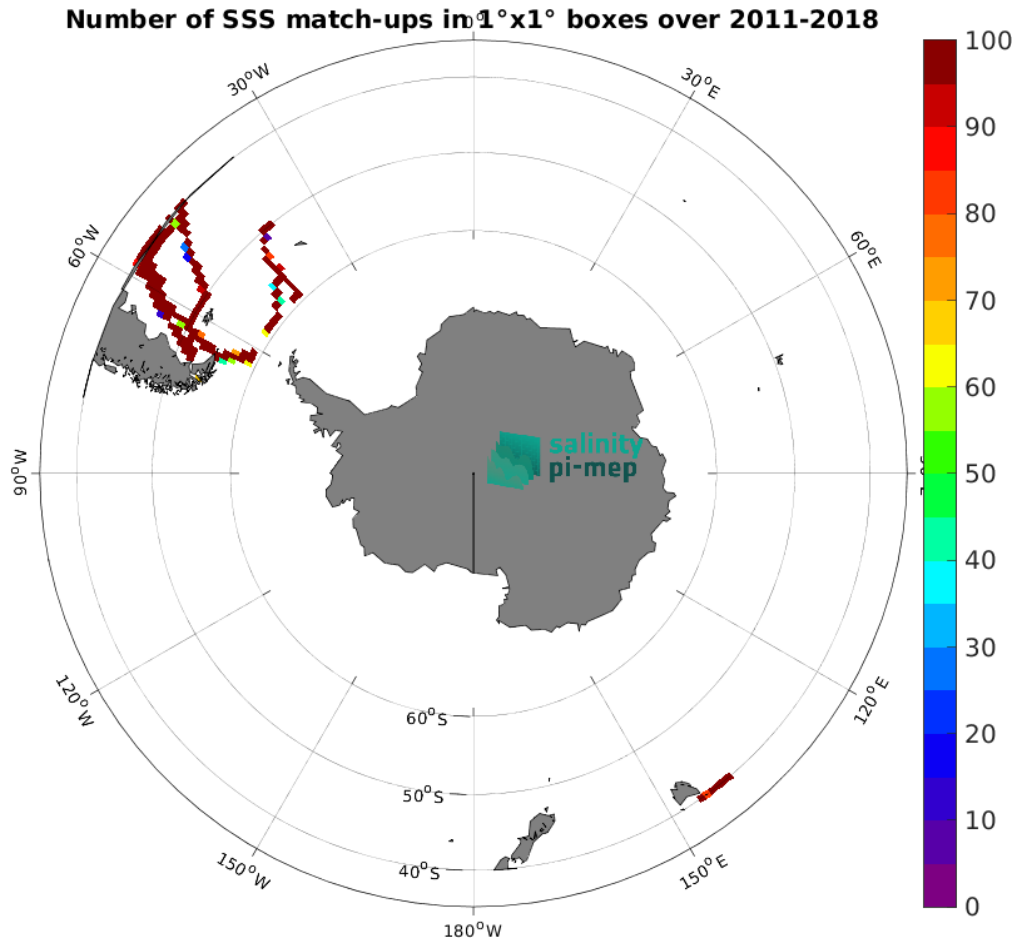
Figure 4: Number of SSS match-ups between TSG (CSIC-UTM) SSS and the SMOS and SMAP SSS L4 OI v1 - 7 Days (LOPS) SSS product for the Roaring Forties and Furious Fifties Pi-MEP region over 1^\circ \times 1^\circ boxes and for the full satellite product period.
