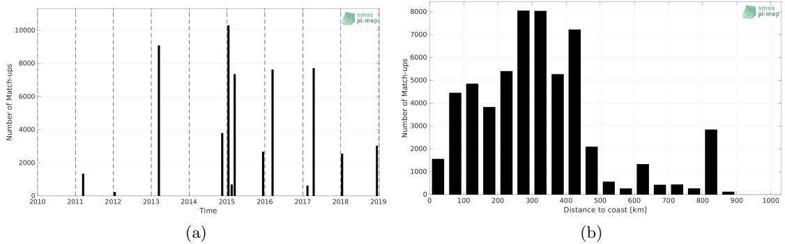
Figure 1: Number of match-ups between TSG (CSIC-UTM) and SMOS and SMAP SSS L4 OI v1 - 7 Days (LOPS) SSS as a function of time (a) and as function of the distance to coast (b) over the Roaring Forties and Furious Fifties Pi-MEP region and for the full satellite product period.
