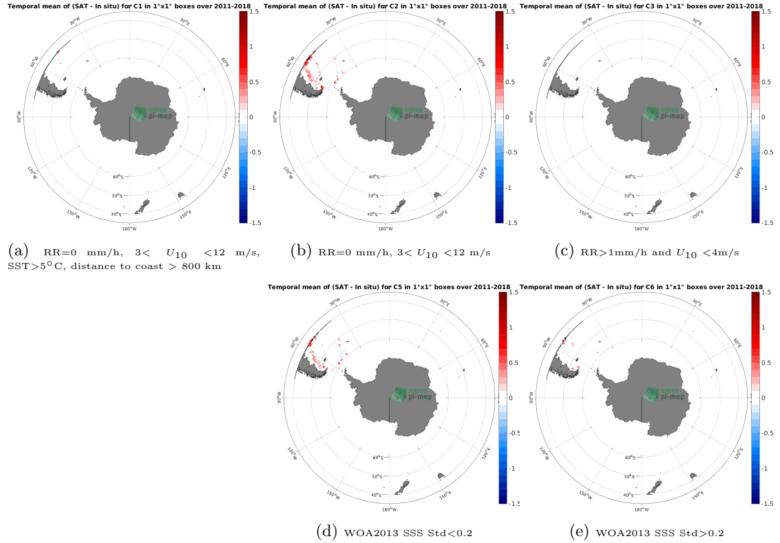
Figure 12: Temporal mean gridded over spatial boxes of size 1^{\circ}\times 1^{\circ} of \Delta\text{SSS} (SMOS and SMAP SSS L4 OI v1 - 7 Days (LOPS) - TSG (CSIC-UTM)) for 5 different subdatasets corresponding to:RR=0 mm/h, 3 < U_{10} < 12 m/s, SST >5^{\circ}\text{C} , distance to coast > 800 km (a), RR=0 mm/h, 3 < U_{10} < 12 m/s (b), RR >1 mm/h and U_{10} < 4 m/s (c), WOA2013 SSS Std <0.2 (d), WOA2013 SSS Std >0.2 (e).
