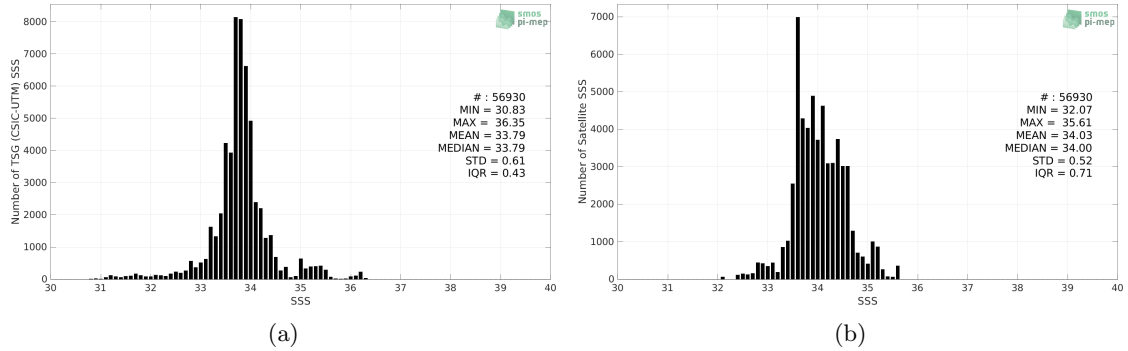
Figure 2: Histograms of SSS from TSG (CSIC-UTM) (a) and SMOS and SMAP SSS L4 OI v1 - 7 Days (LOPS) (b) considering all match-up pairs per bins of 0.1 over the Roaring Forties and Furious Fifties Pi-MEP region and for the full satellite product period.
