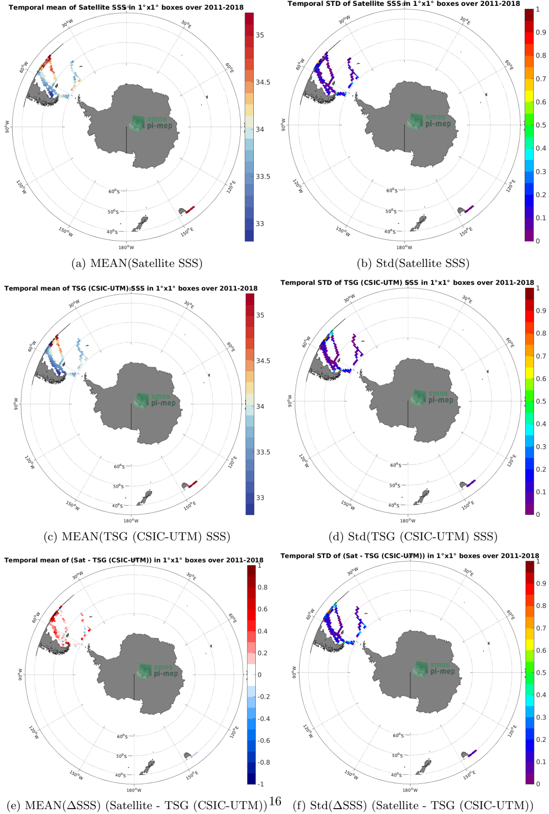
Figure 6: Temporal mean (left) and Std (right) of SSS from SMOS and SMAP SSS L4 OI v1 - 7 Days (LOPS) (top), TSG (CSIC-UTM) (middle), and of \Delta SSS (Satellite - TSG (CSIC-UTM)). Only match-up pairs are used to generate these maps.
