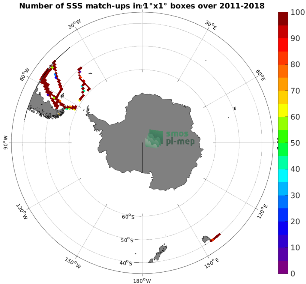
Figure 4: Number of SSS match-ups between TSG (CSIC-UTM) SSS and the SMOS and SMAP SSS L4 OI v1 - 7 Days (LOPS) SSS product for the Roaring Forties and Furious Fifties Pi-MEP region over 1^\circ \times 1^\circ boxes and for the full satellite product period.
