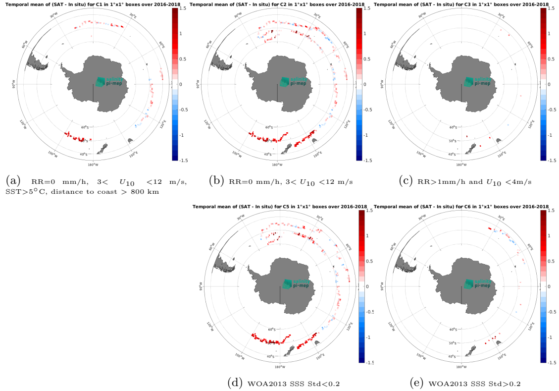
Figure 11: Temporal mean gridded over spatial boxes of size 1^{\circ}\times 1^{\circ} of \Delta\text{SSS} (SMOS and SMAP SSS L4 OI v1 - 7 Days (LOPS) - Surface drifters) for 5 different subdatasets corresponding to:RR=0 mm/h, 3 < U_{10} < 12 m/s, SST >5^{\circ}\text{C} , distance to coast > 800 km (a), RR=0 mm/h, 3 < U_{10} < 12 m/s (b), RR >1 mm/h and U_{10} < 4 m/s (c), WOA2013 SSS Std <0.2 (d), WOA2013 SSS Std >0.2 (e).
