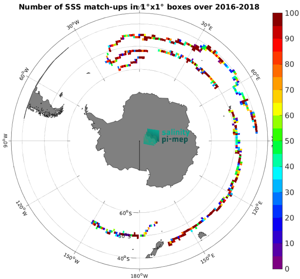
Figure 3: Number of SSS match-ups between Surface drifters SSS and the SMOS and SMAP SSS L4 OI v1 - 7 Days (LOPS) SSS product for the Roaring Forties and Furious Fifties Pi-MEP region over 1^\circ \times 1^\circ boxes and for the full satellite product period.
