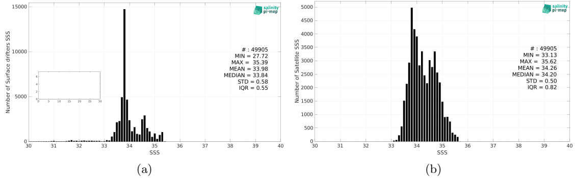
Figure 2: Histograms of SSS from Surface drifters (a) and SMOS and SMAP SSS L4 OI v1 - 7 Days (LOPS) (b) considering all match-up pairs per bins of 0.1 over the Roaring Forties and Furious Fifties Pi-MEP region and for the full satellite product period.
