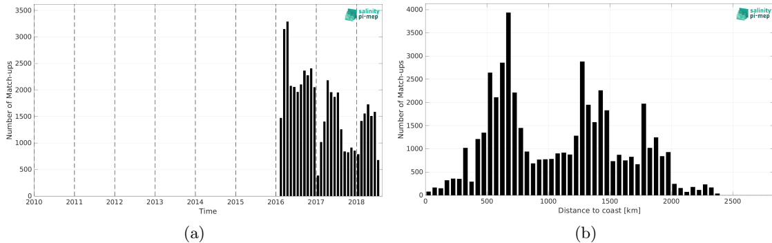
Figure 1: Number of match-ups between Surface drifters and SMOS and SMAP SSS L4 OI v1 - 7 Days (LOPS) SSS as a function of time (a) and as function of the distance to coast (b) over the Roaring Forties and Furious Fifties Pi-MEP region and for the full satellite product period.
