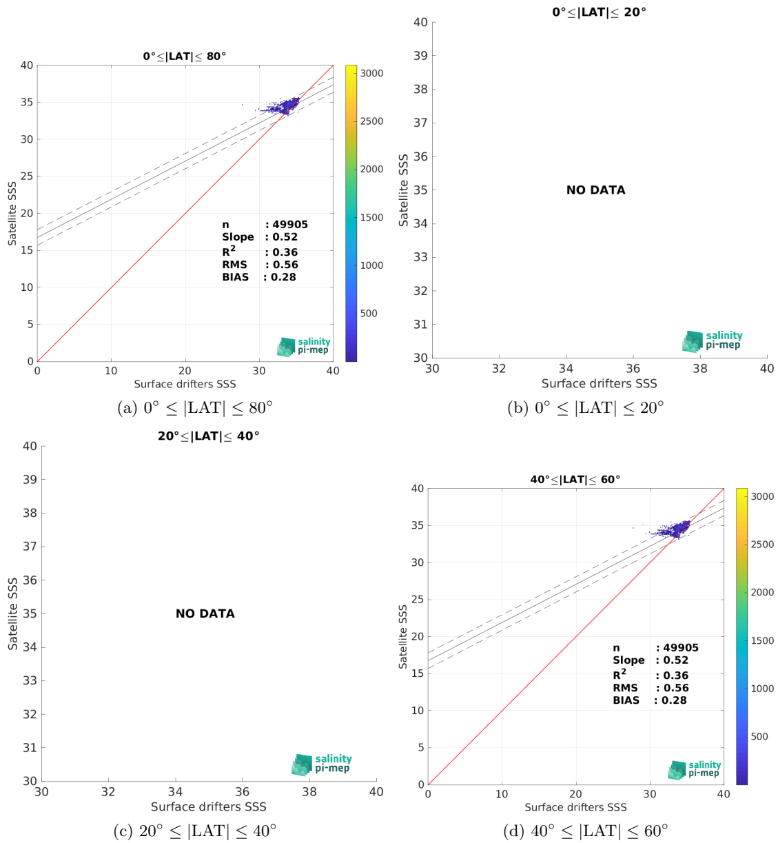
Figure 8: Contour maps of the concentration of SMOS and SMAP SSS L4 OI v1 - 7 Days (LOPS) SSS (y-axis) versus Surface drifters SSS (x-axis) at match-up pairs for different latitude bands. For each plot, the red line shows x=y . The black thin and dashed lines indicate a linear fit through the data cloud and the \pm 95\% confidence levels, respectively. The number match-up pairs n , the slope and R^2 coefficient of the linear fit, the root mean square (RMS) and the mean bias between satellite and in situ data are indicated for each latitude band in each plots.
