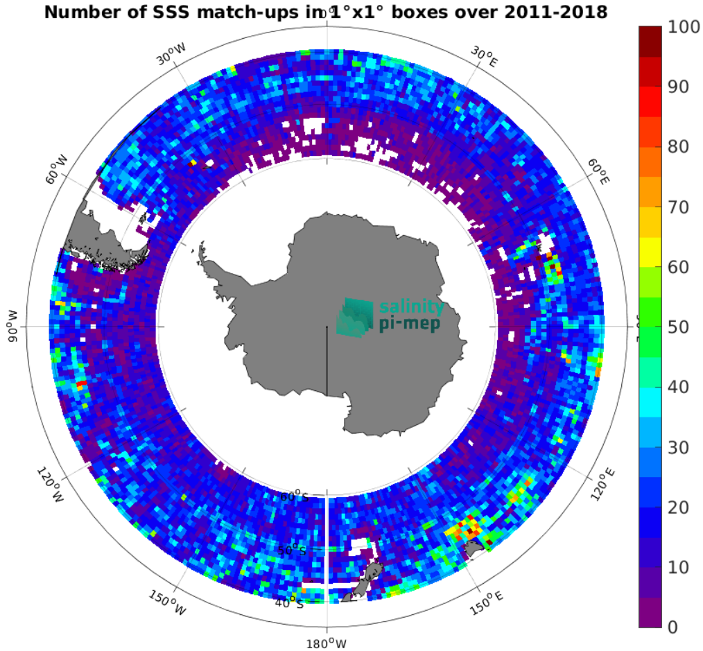
Figure 4: Number of SSS match-ups between Argo SSS and the SMOS and SMAP SSS L4 OI v1 - 7 Days (LOPS) SSS product for the Roaring Forties and Furious Fifties Pi-MEP region over 1^\circ \times 1^\circ boxes and for the full satellite product period.
