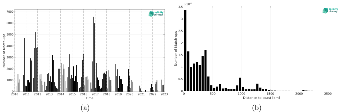
Figure 1: Number of match-ups between TSG (SAMOS) and SMOS SSS L4 v1 - Weekly (CMEMS-CNR) SSS as a function of time (a) and as function of the distance to coast (b) over the Roaring Forties and Furious Fifties Pi-MEP region and for the full satellite product period.
