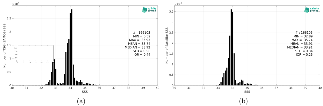
Figure 2: Histograms of SSS from TSG (SAMOS) (a) and SMOS SSS L4 v1 - Weekly (CMEMS-CNR) (b) considering all match-up pairs per bins of 0.1 over the Roaring Forties and Furious Fifties Pi-MEP region and for the full satellite product period.
